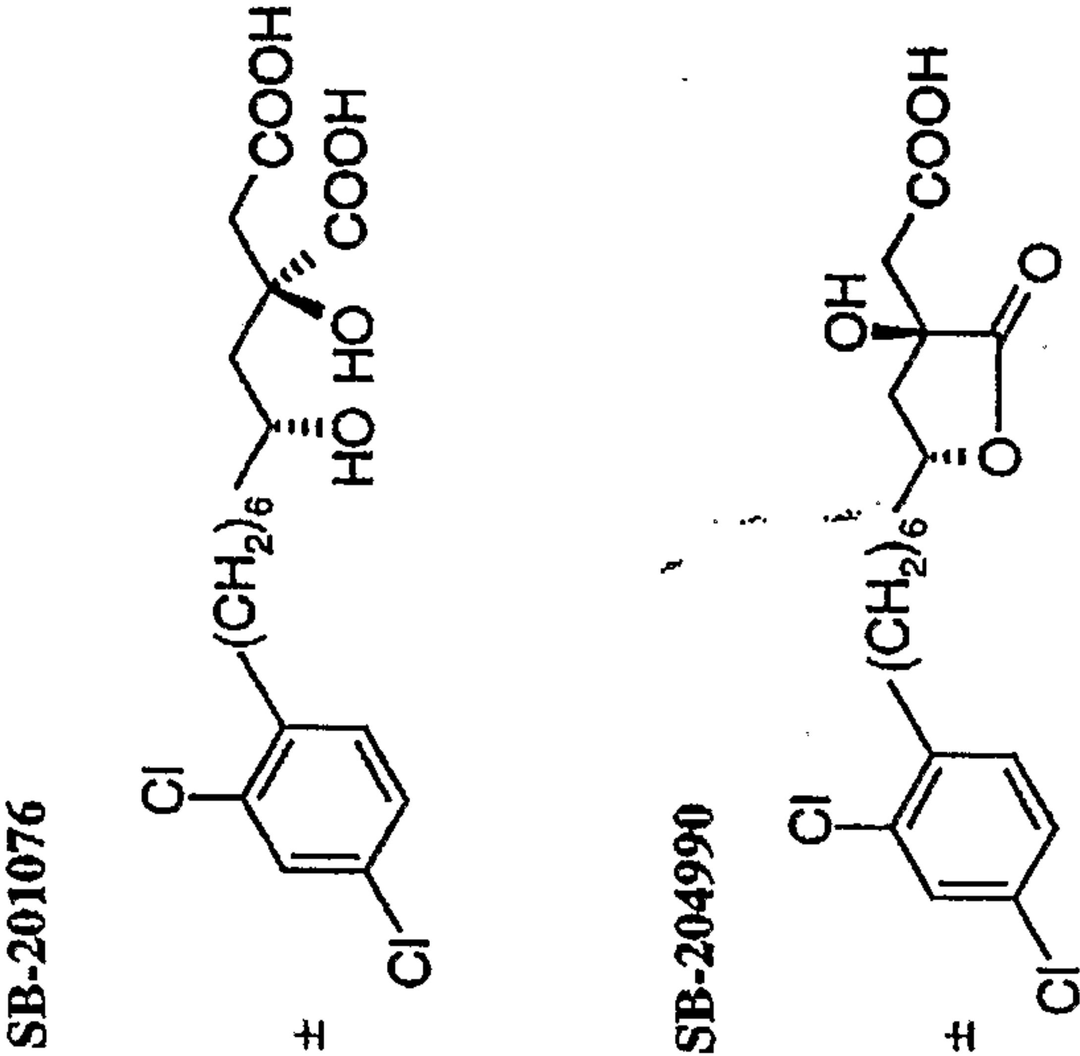
Figure 1 Structure of SB-201076 and its \gamma -lactone SB-204990
