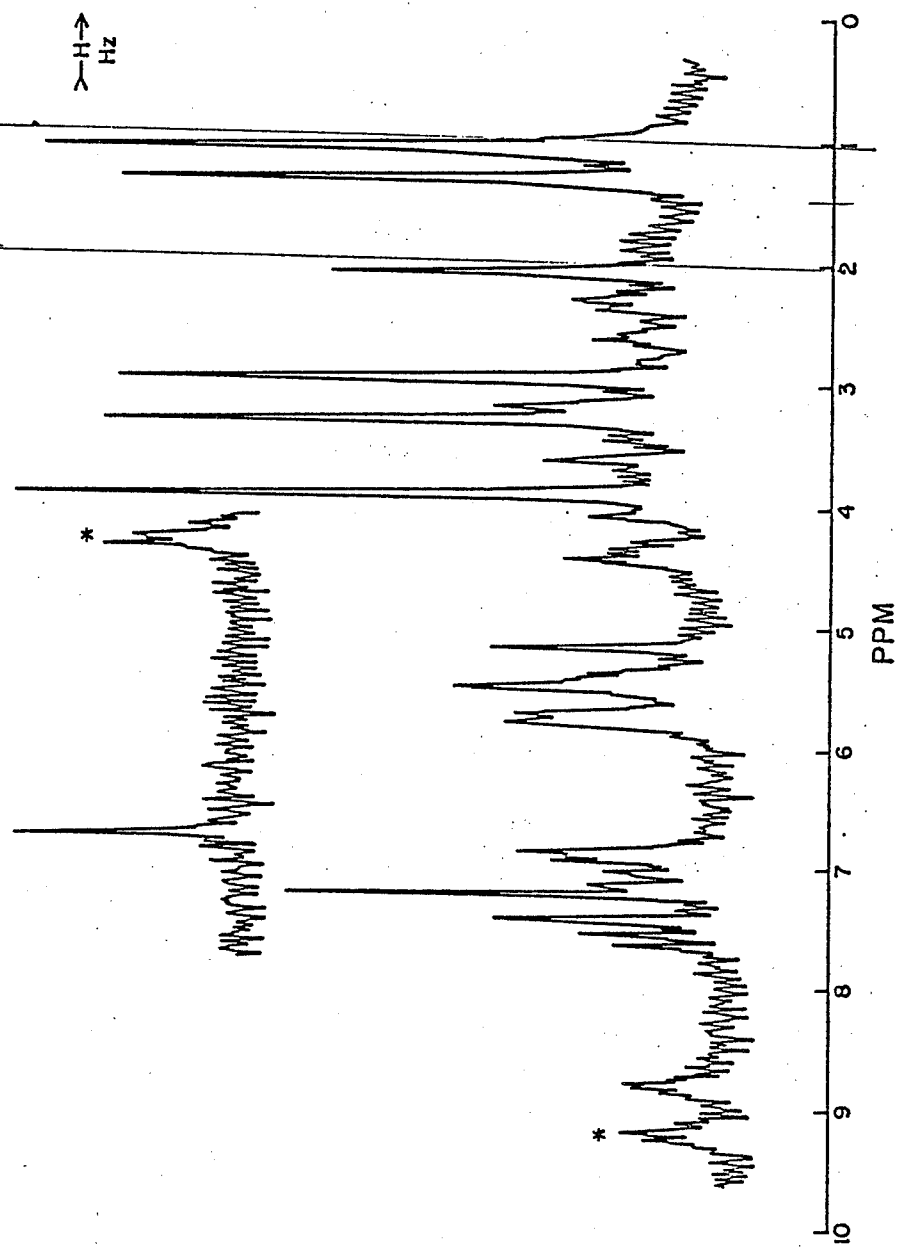
FIG. 8 NMR SPECTRUM OF BBM-928 D
