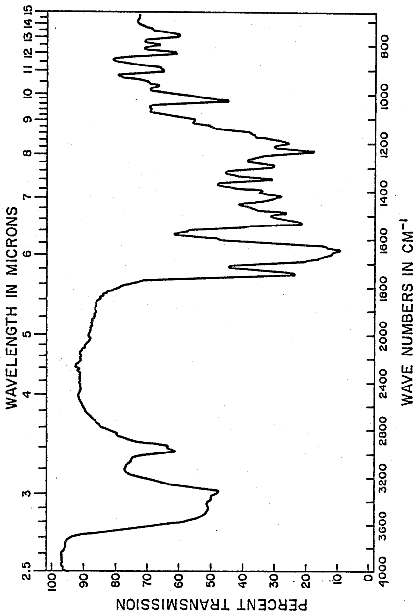
FIG. 4 INFRARED SPECTRUM OF BBM-928 D
