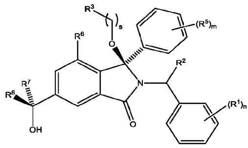
Diastereoisomer 2B
