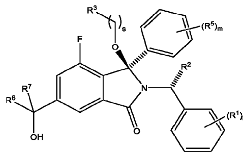
Diastereoisomer 1B
