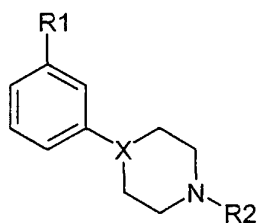
Formula II
