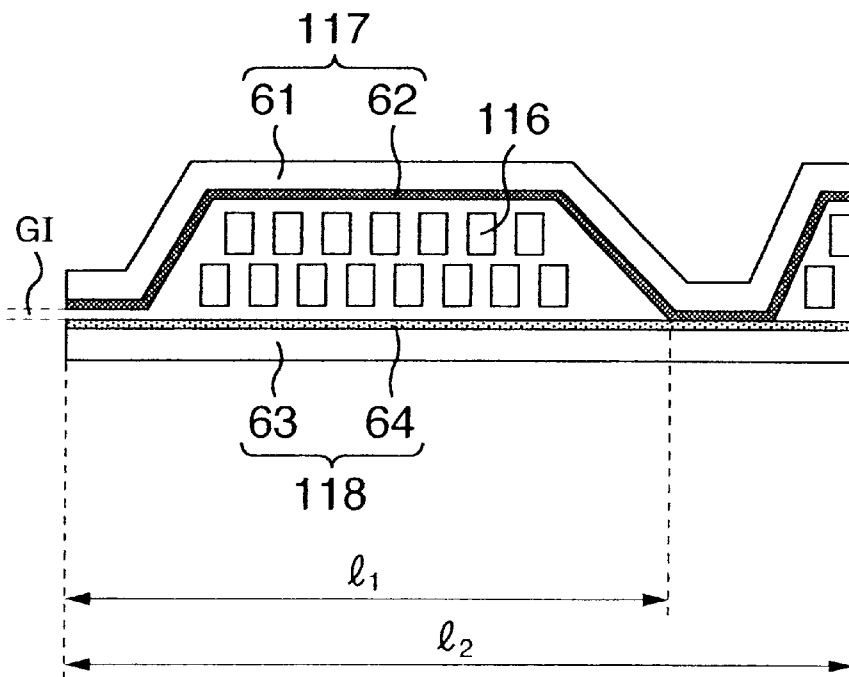
CROSS SECTION
