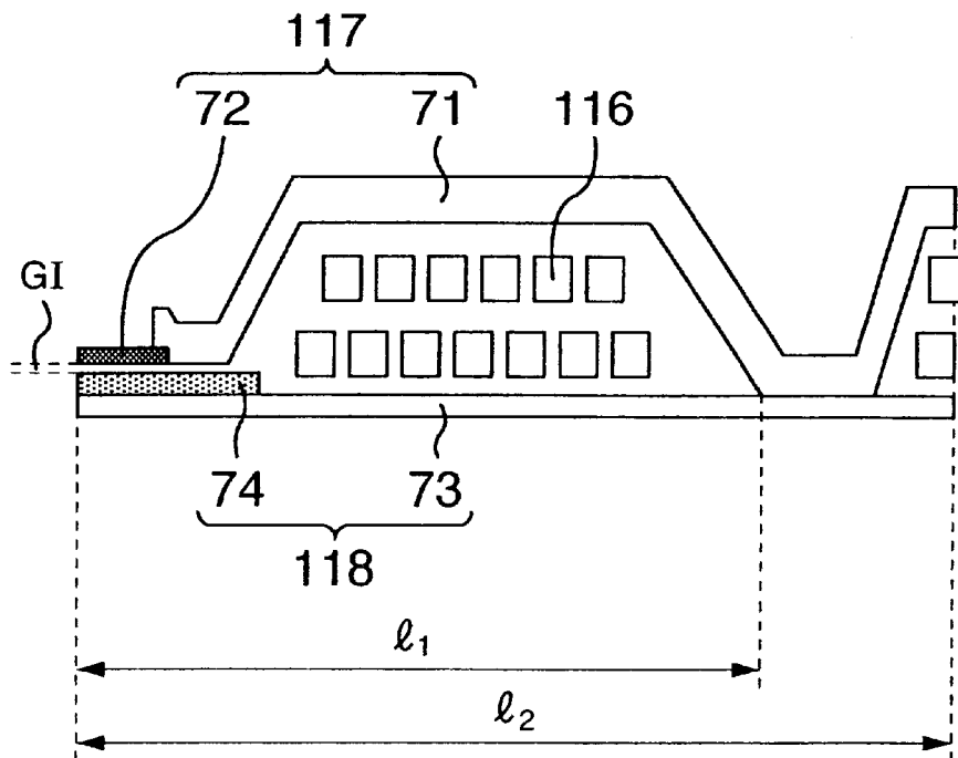
CROSS SECTION
