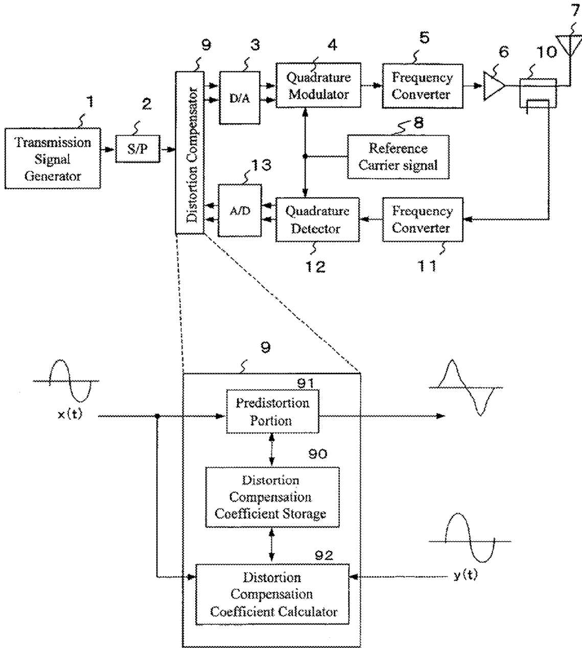
FIG. 4 (RELATED ART)
