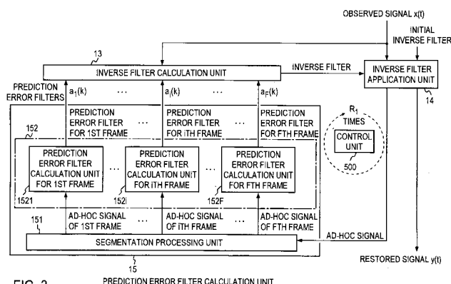
FIG. 3 PREDICTION ERROR FILTER CALCULATION UNIT
