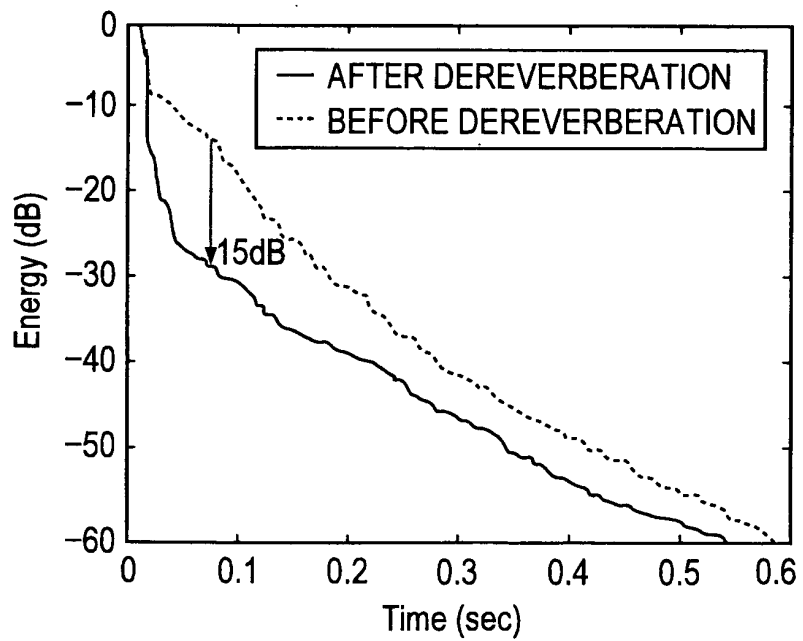
EXAMPLE OF ENERGY DECAY CURVE BEFORE AND AFTER DEREVERBERATION
