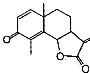
3-KETO-EUDISM-1(2), 4(5), 11(13)-TRIENE-6-12-OLID 18
