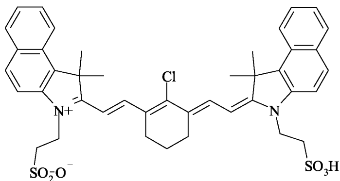
dye I
