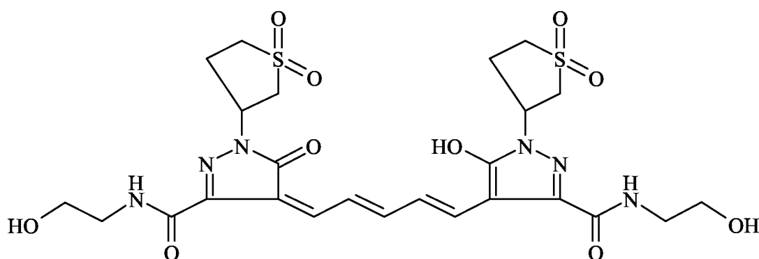
dye II
