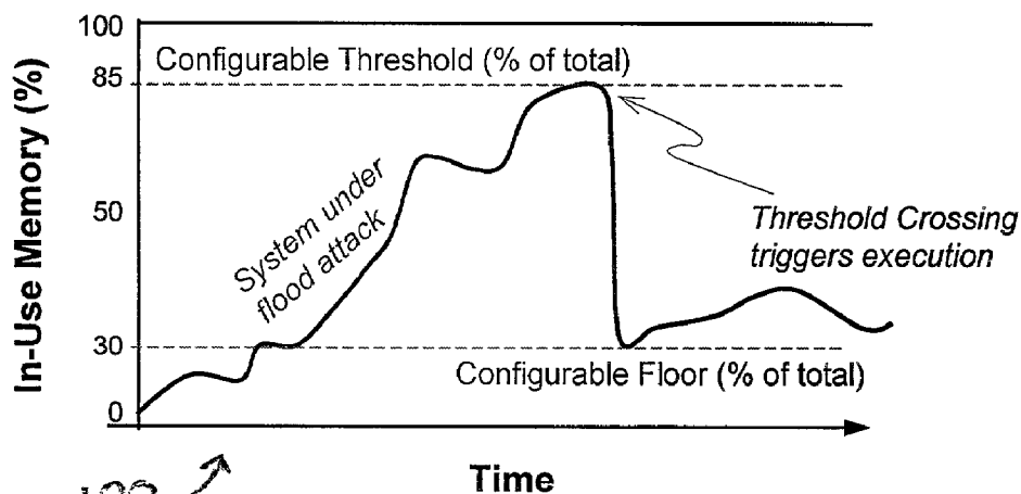
Figure 1. Memory versus time for a system configured to use ICM.
