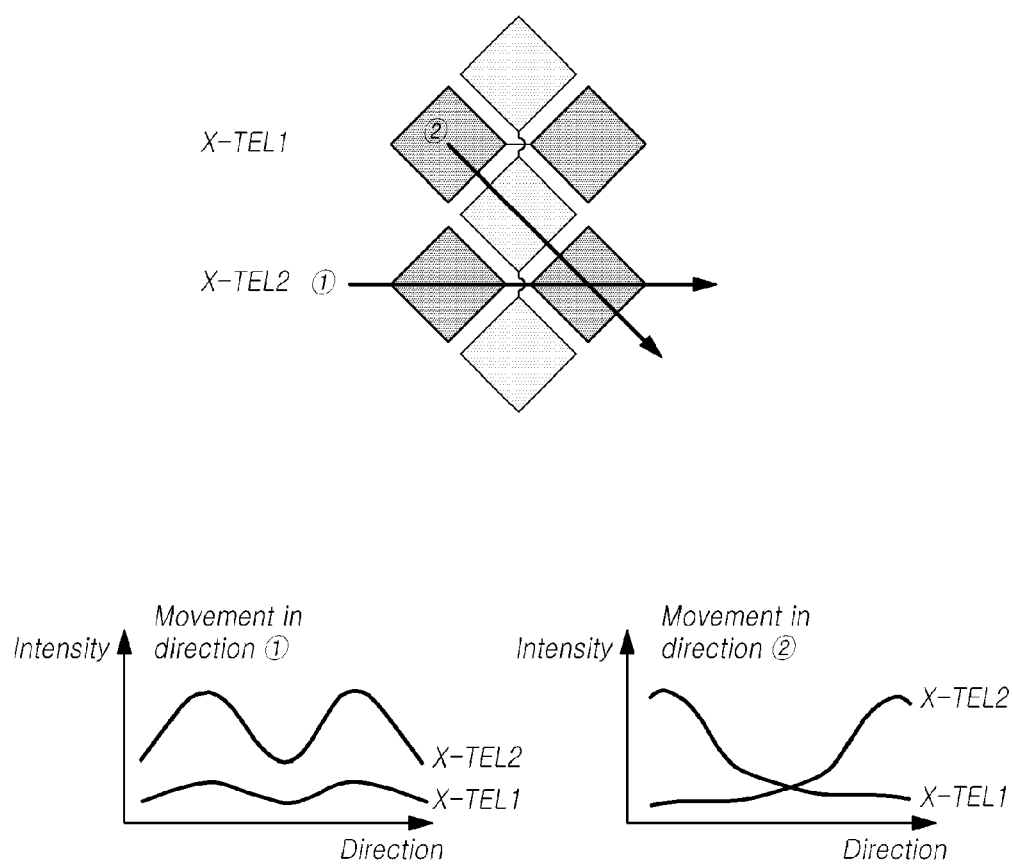
Graph for amount of change in intensity depending on direction in X-TELs
