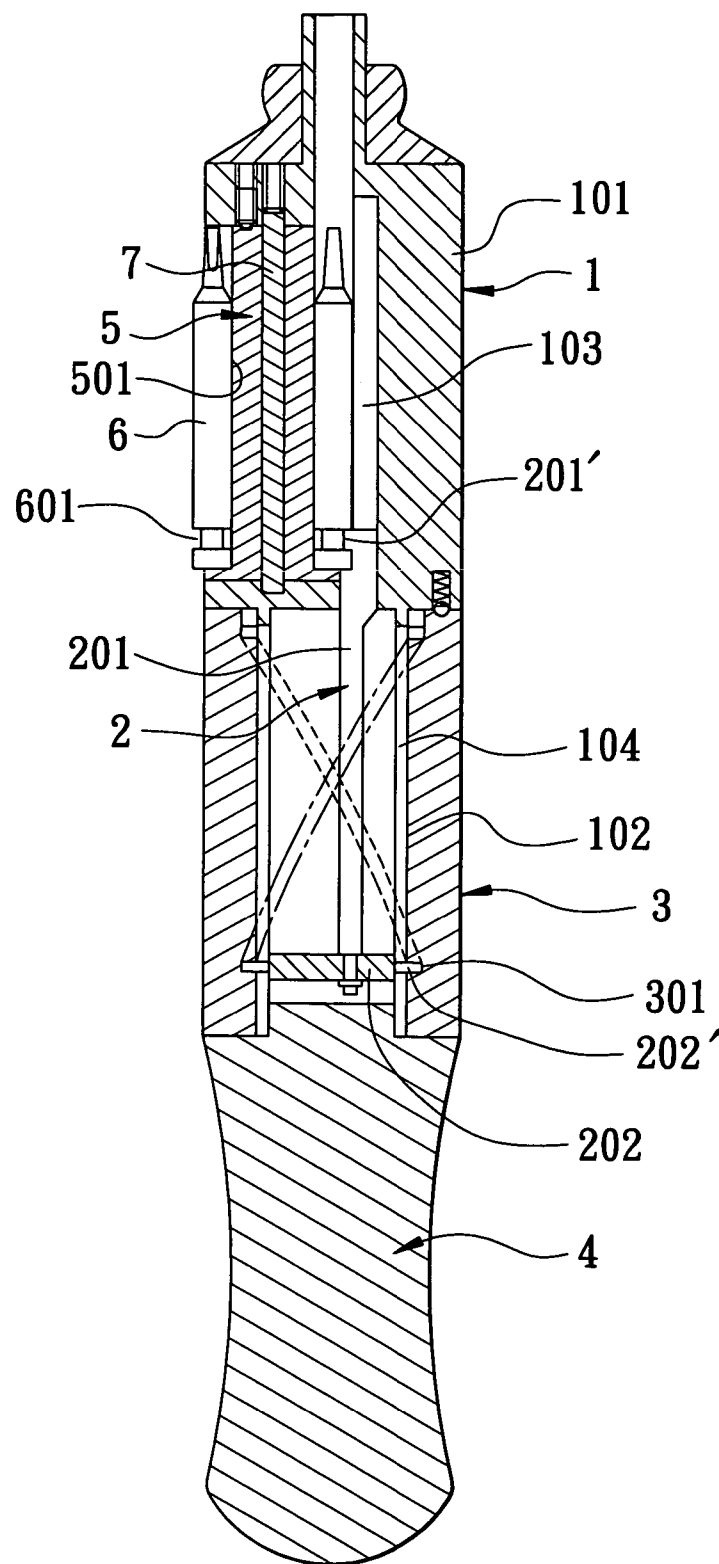
FIG. 2 PRIOR ART
