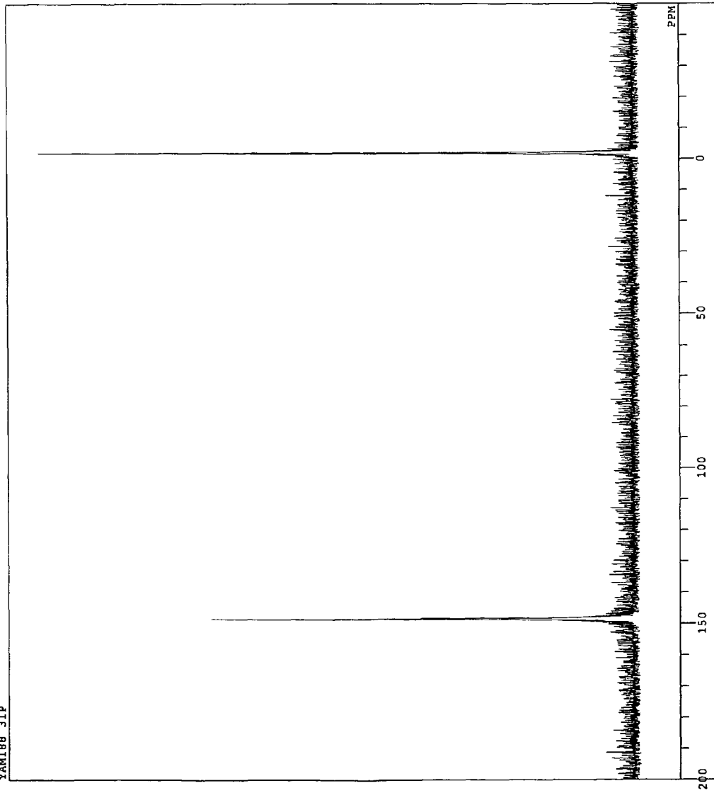
C:\Documents and Settings\JBOL\ffxfNfgfbfv\g'\daglu\dagluP(IV)aramidite 31P.als YAM188_31P FIG.33
