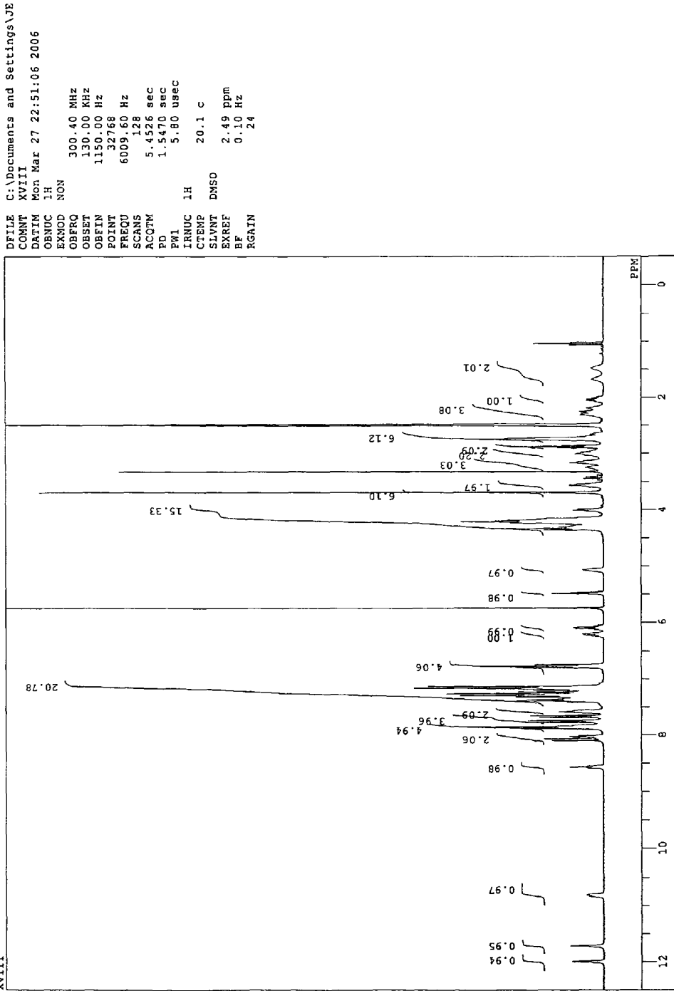
FIG. 39 C:\Documents and Settings\JEOL\ffxfnfbfv\je\dglys\dglysp(V).dcoH 20060327.a1s XVIII
