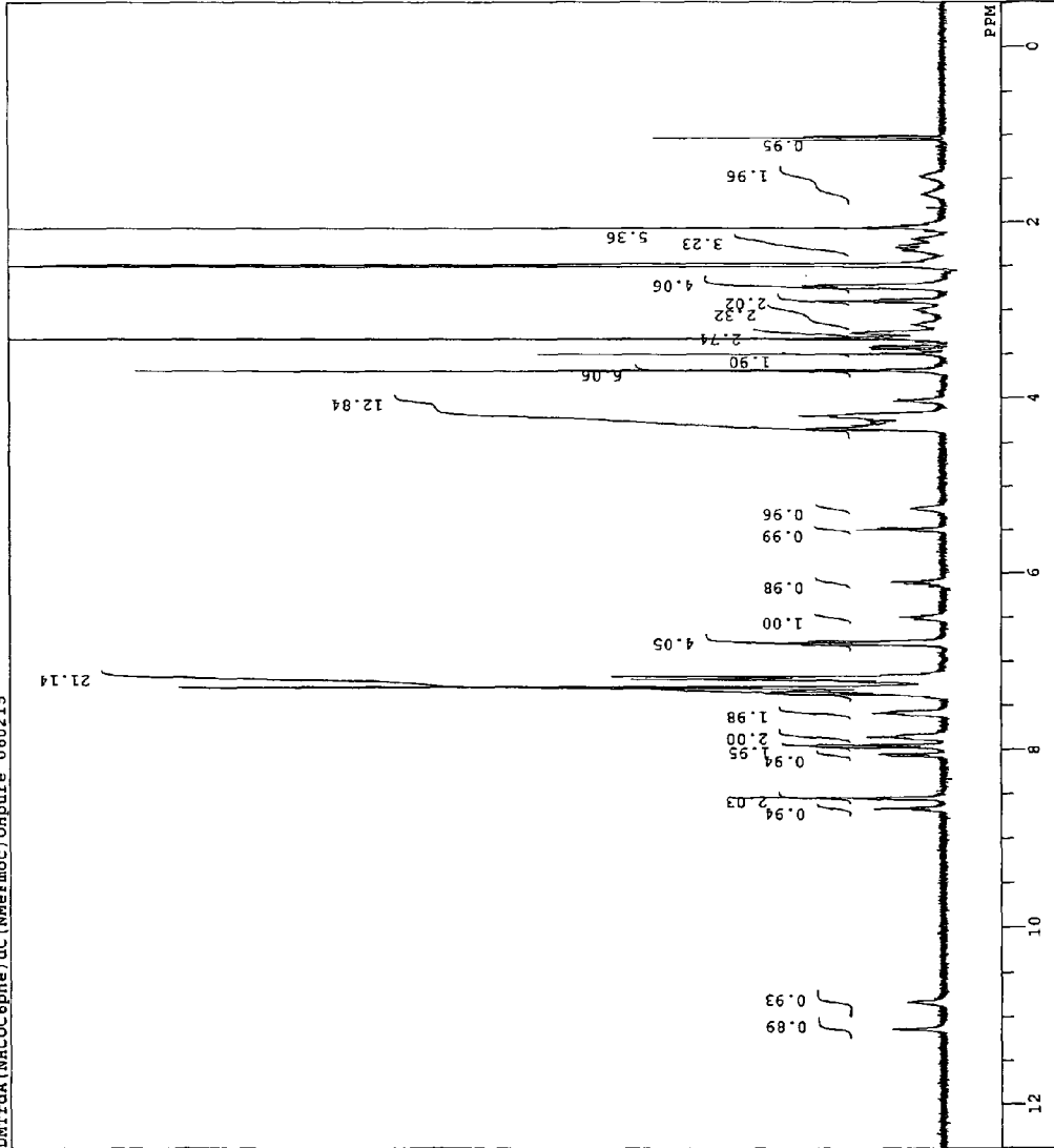
FIG. 24 C:\Documents and Settings\JEOL\jefjfnfjfv\j\g\daphe\DMTrdA(C6phe)P(V) dC (NMeFmoc) OHpure 060215.ais DMTrdA (NHCOC6phe) dC (NMeFmoc) OHpure 060215
