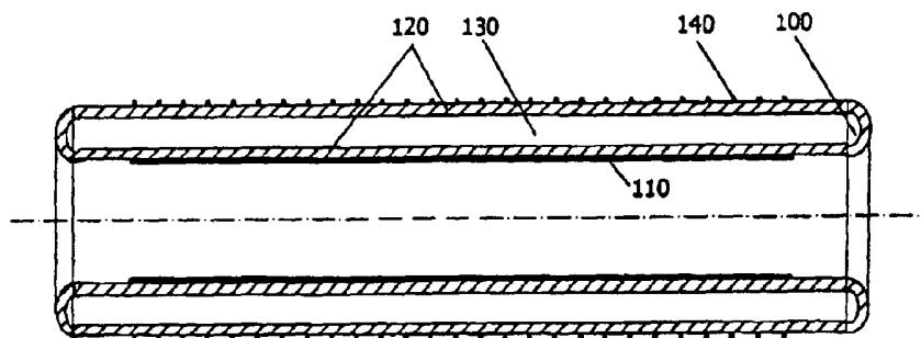
side-on view of typical co-axial DBD lamp
