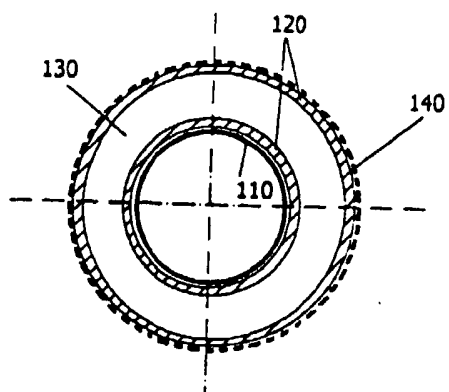
end-on view of typical co-axial DBD lamp
