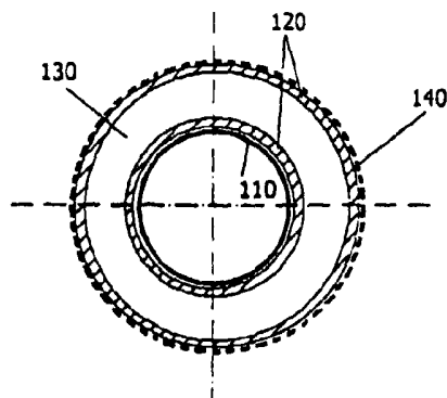
end-on view of typical co-axial DBD lamp
