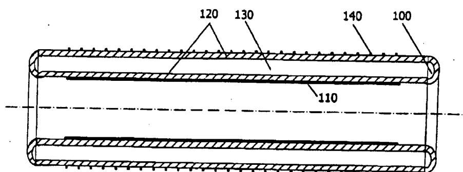
side-on view of typical co-axial DBD lamp
