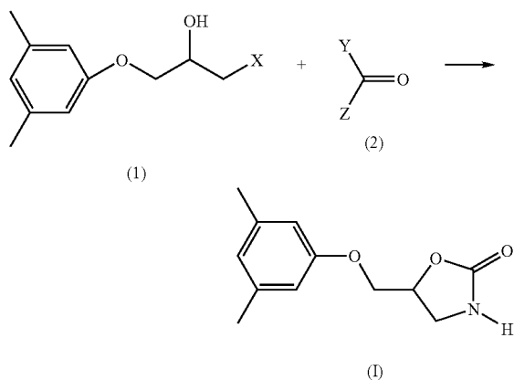
Scheme-1: Method for preparation of Metaxalone
