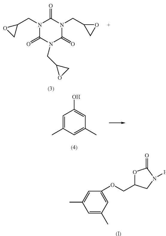
Scheme-2: Method for preparation of Metaxalone
