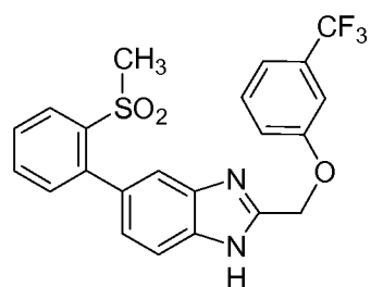
Cpd 75
