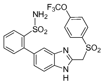
Cpd 46
