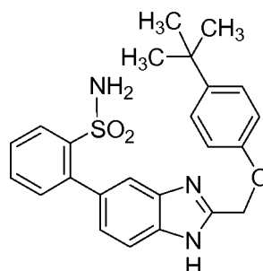
Cpd 32
