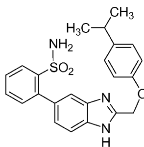
Cpd 28
