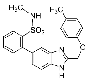
Cpd 17
