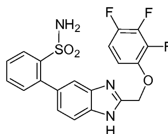
Cpd 14
