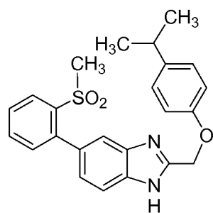
Cpd 77
