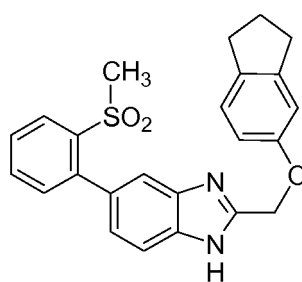
Cpd 91
