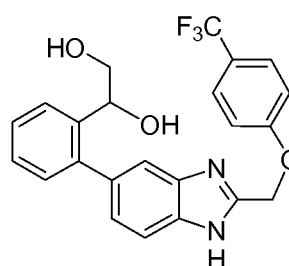
Cpd 150
