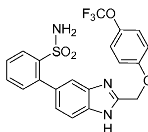
Cpd 16
