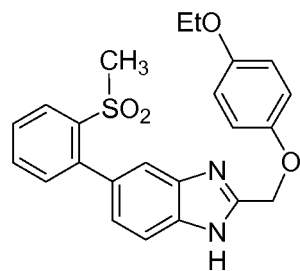
Cpd 81
