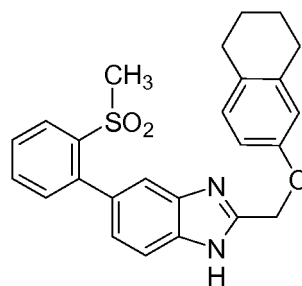
Cpd 85
