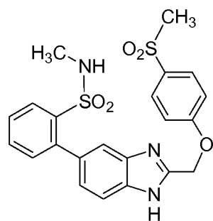
Cpd 19
