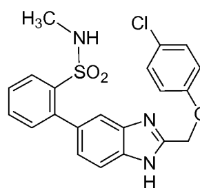
Cpd 18
