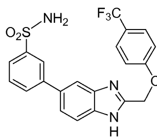
Cpd 104
