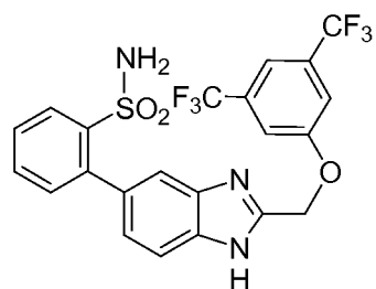
Cpd 31
