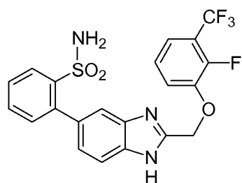
Cpd 71
