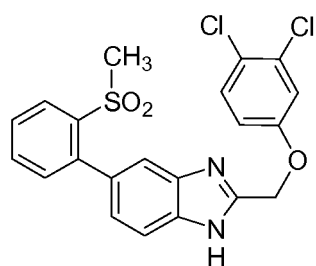
Cpd 65
