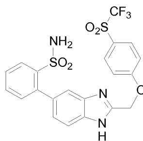
Cpd 2
