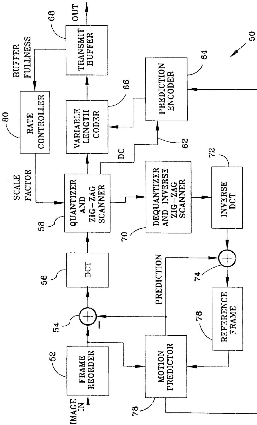
Fig. 4 (PRIOR ART)
