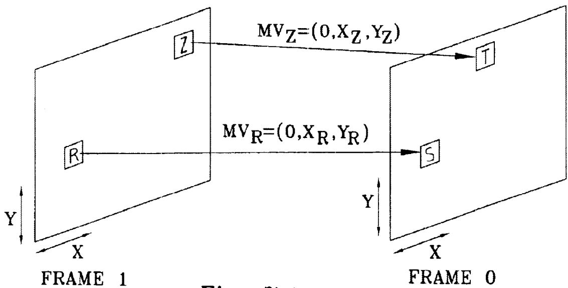
Fig. 7 (PRIOR ART)
