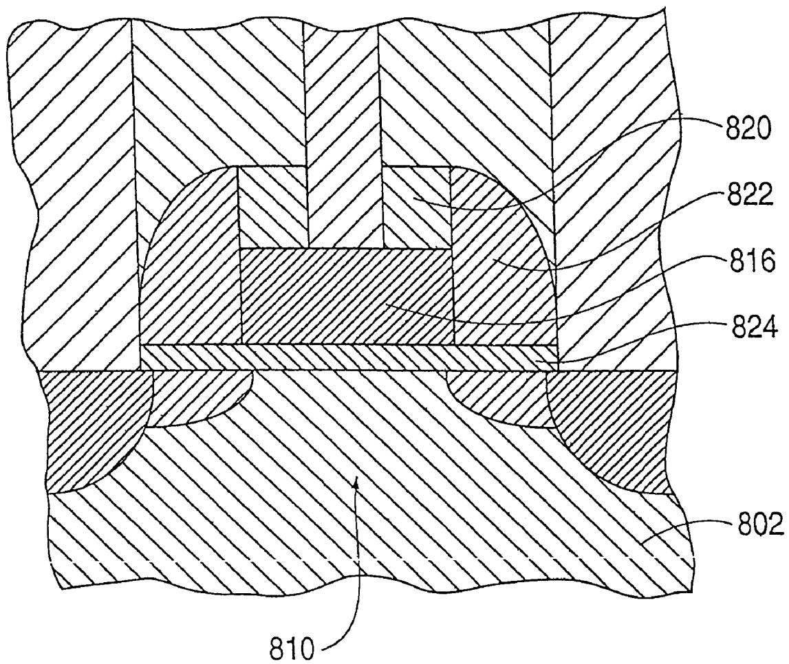
FIG. 23 (PRIOR ART)
