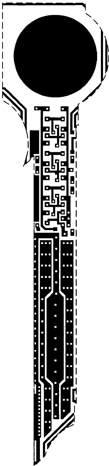
Metal 1 mask
