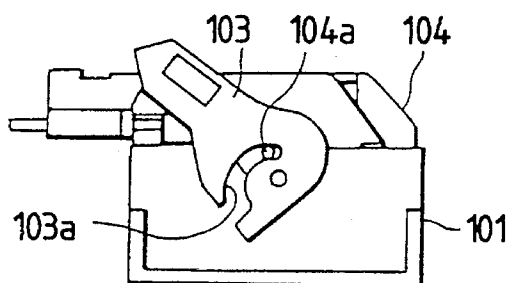
FIG. 17C PRIOR ART
