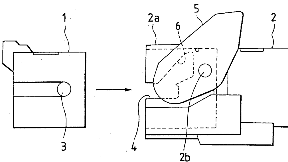
FIG. 14 PRIOR ART
