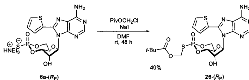
Scheme 11
