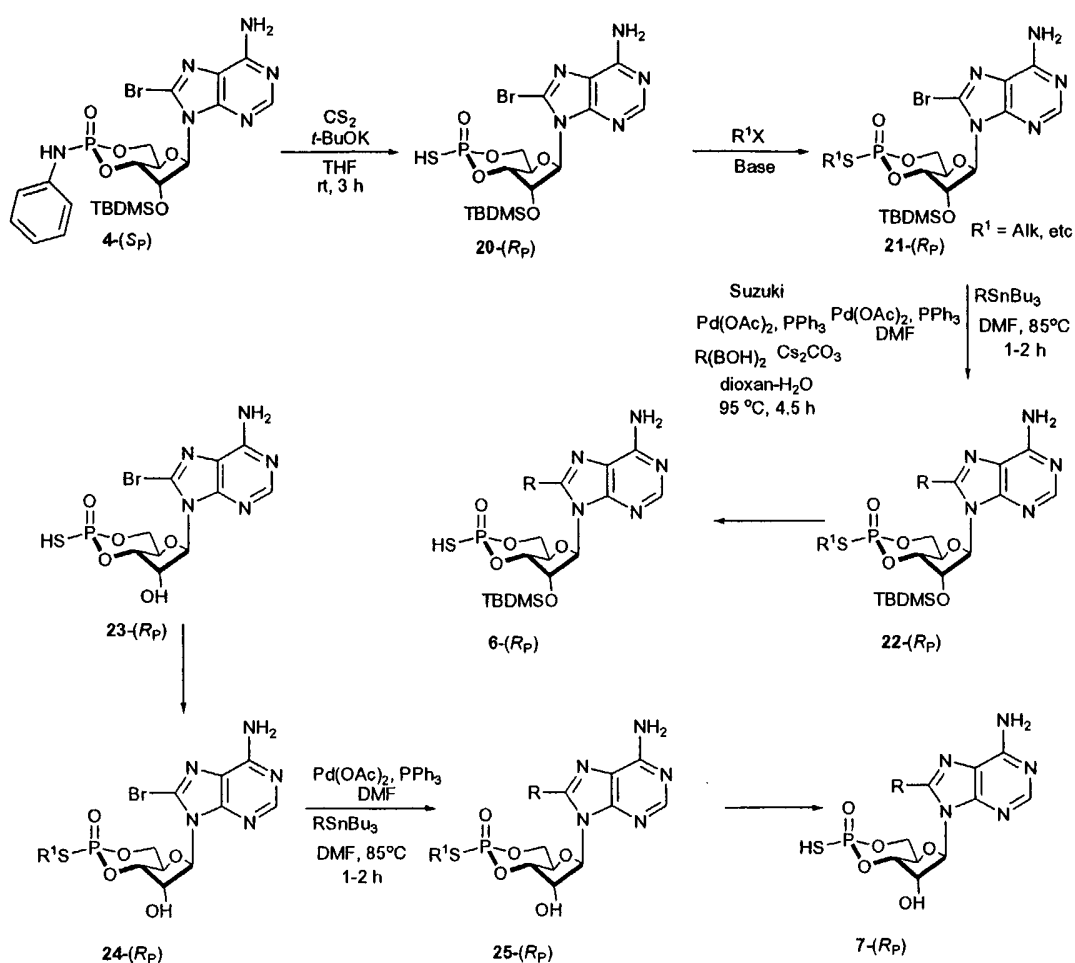
Scheme 10
