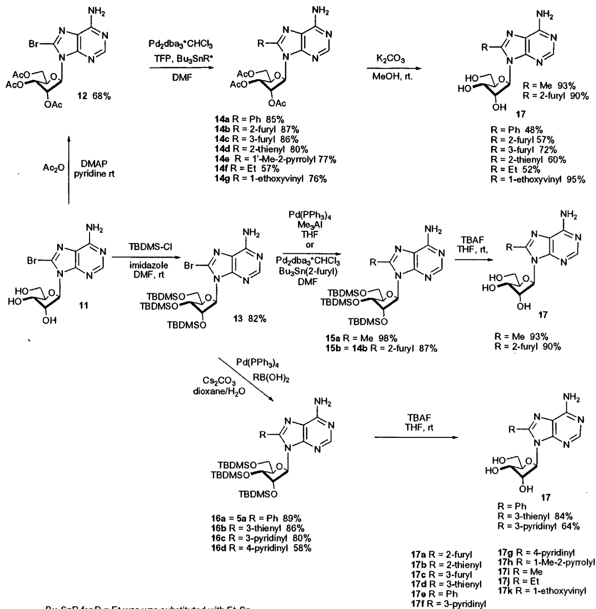
Scheme 7
