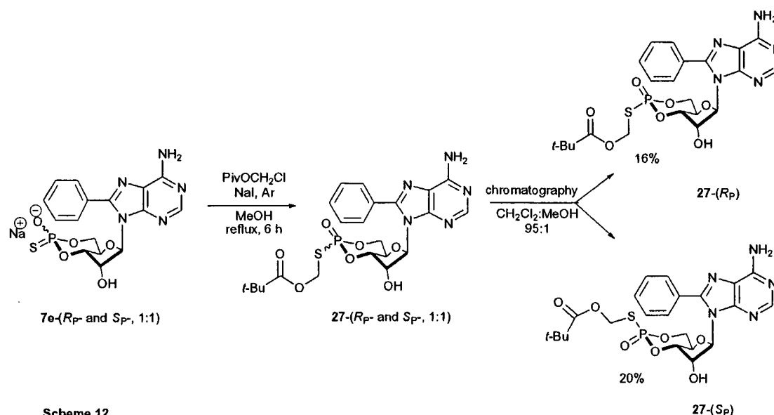
Scheme 12
