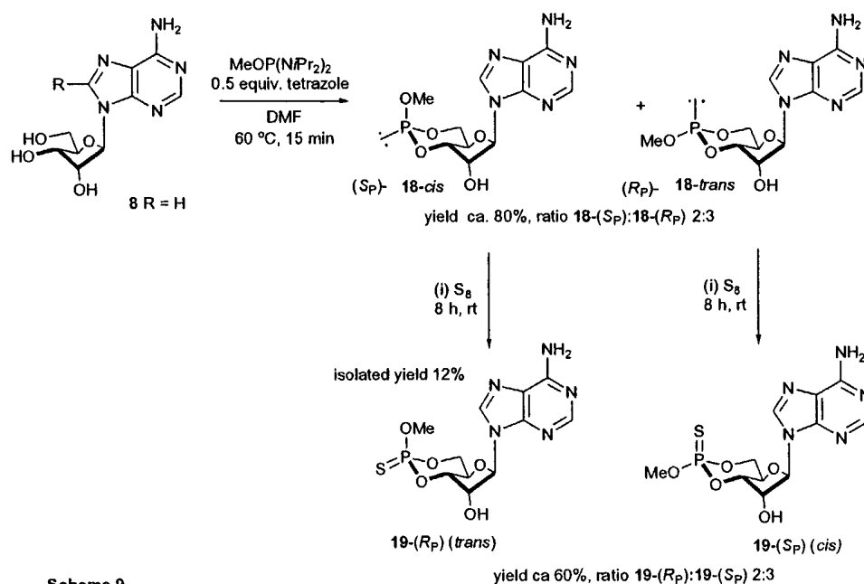
Scheme 9
