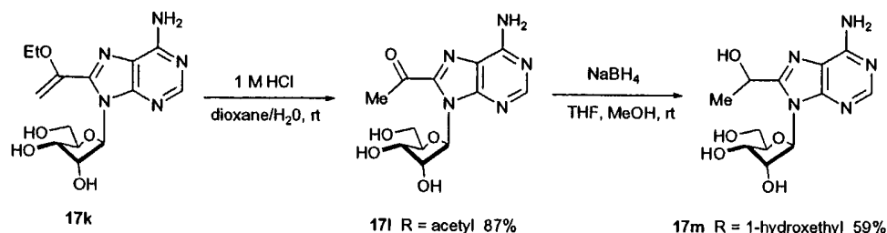
Scheme 8
