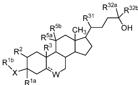
Formula SIX.
