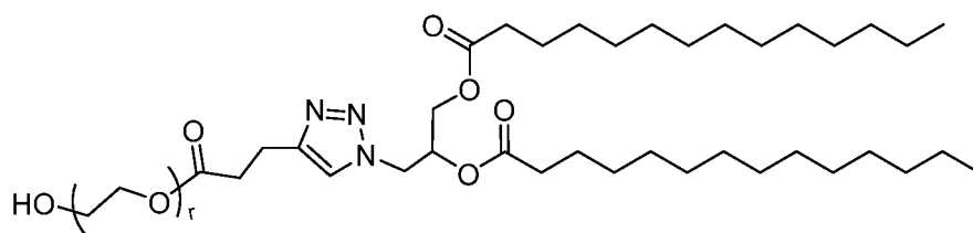
(Compound P-415A),
