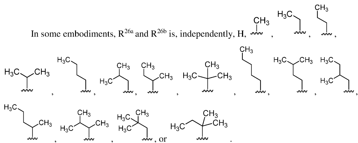
Formula SVIIb,
