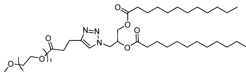
(Compound P-416)
