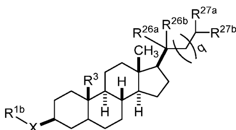
Formula SVIIb,
