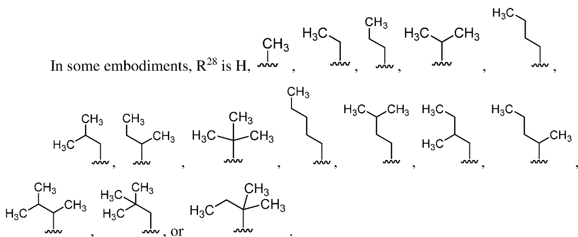
Formula SVIIIb,
