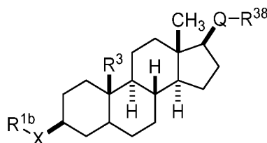
Formula SXIIb,
