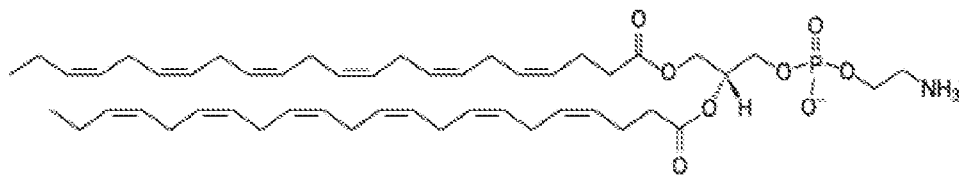
22:6PE;
