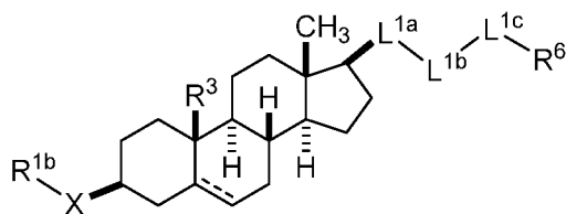
Formula 1d,
