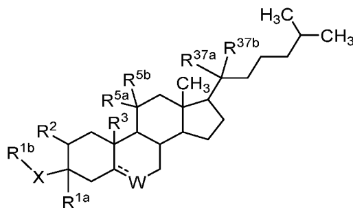
Formula SXI,
