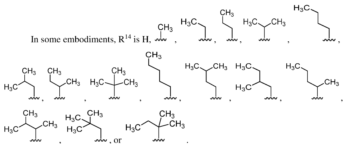
Formula IIIb,
