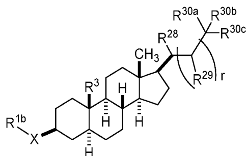
Formula SVIIIb,
