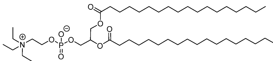
(Compound H-401);
