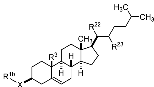
Formula SVa,
