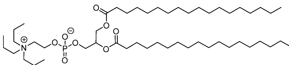
(Compound H-403);
