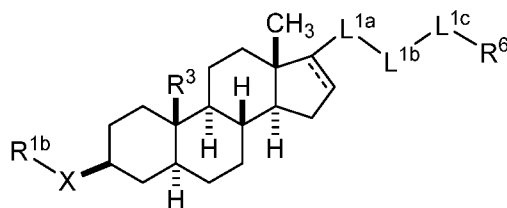
Formula SIb,
