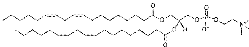
(PC(18:2(9Z,12Z)/18:2(9Z,12Z));
