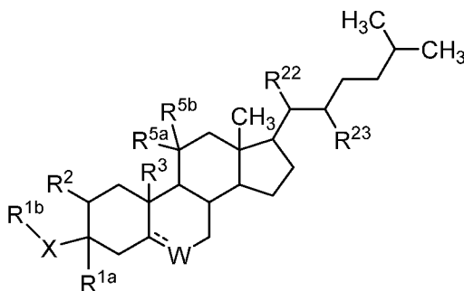
Formula SV,
