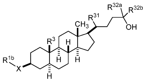
Formula SIXb,
