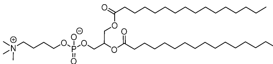
(Compound H-413)
