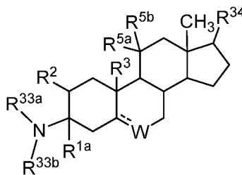
Formula SX,
