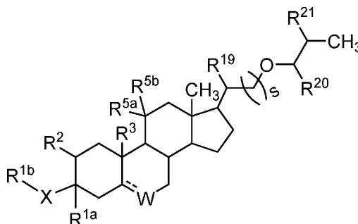
Formula SIV,
