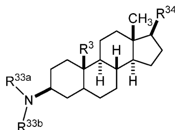
Formula SXb,
