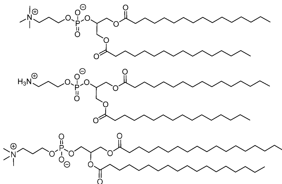
(Compound H-411)
