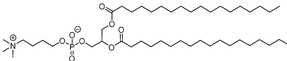
(Compound H-414),
