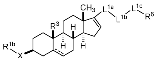
Formula 1c,
