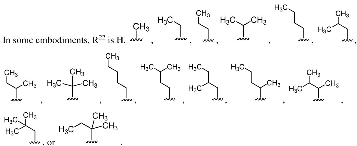
Formula SVb,
