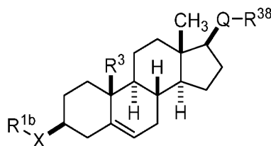
Formula SXIIa,
