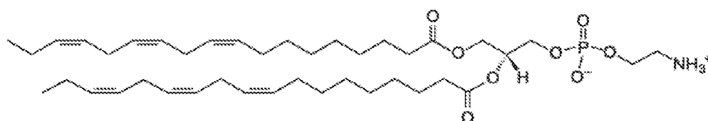
PE (18:3(9Z,12Z,15Z)/18:3(9Z,12Z,15Z));
