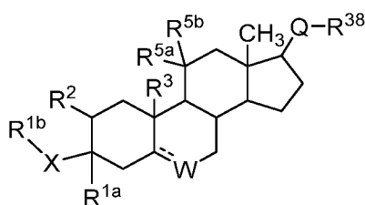
Formula SXII,
