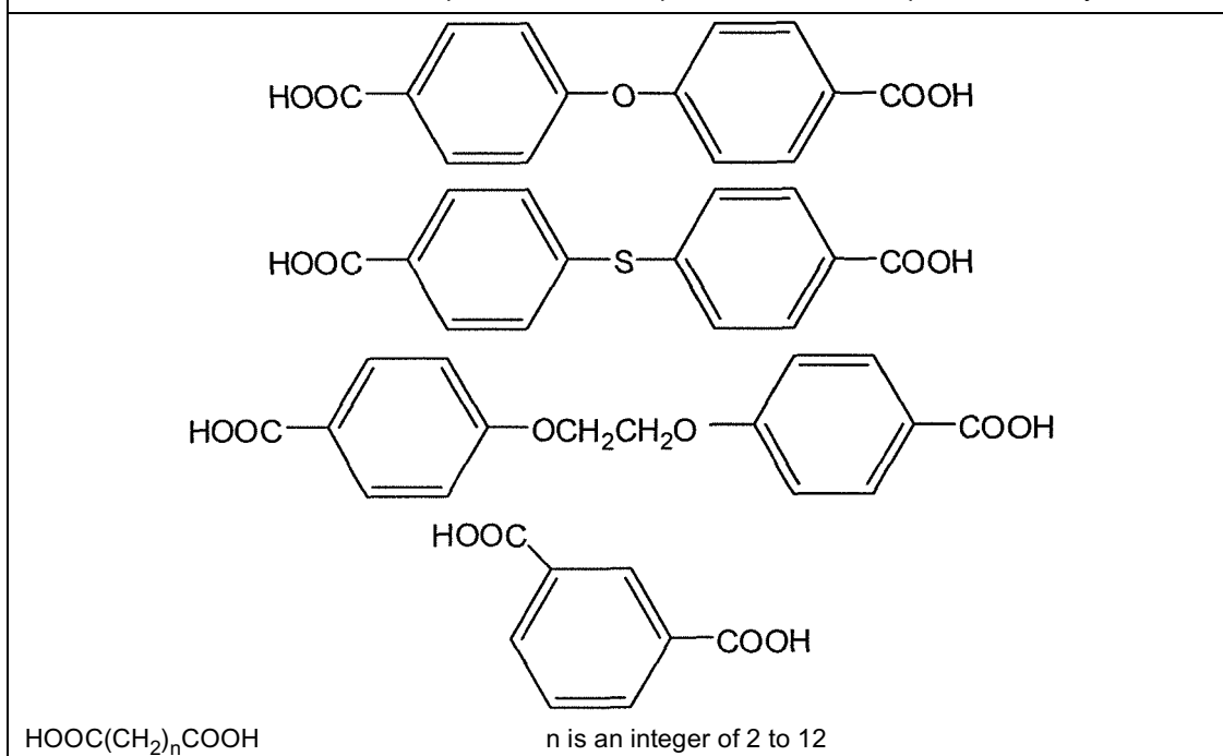
Chemical structural formulae of representative examples of aromatic or aliphatic dicarboxylic acids
