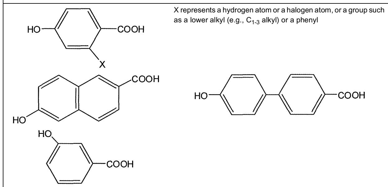
Chemical structural formulae of representative examples of aromatic or aliphatic hydroxycarboxylic acids
