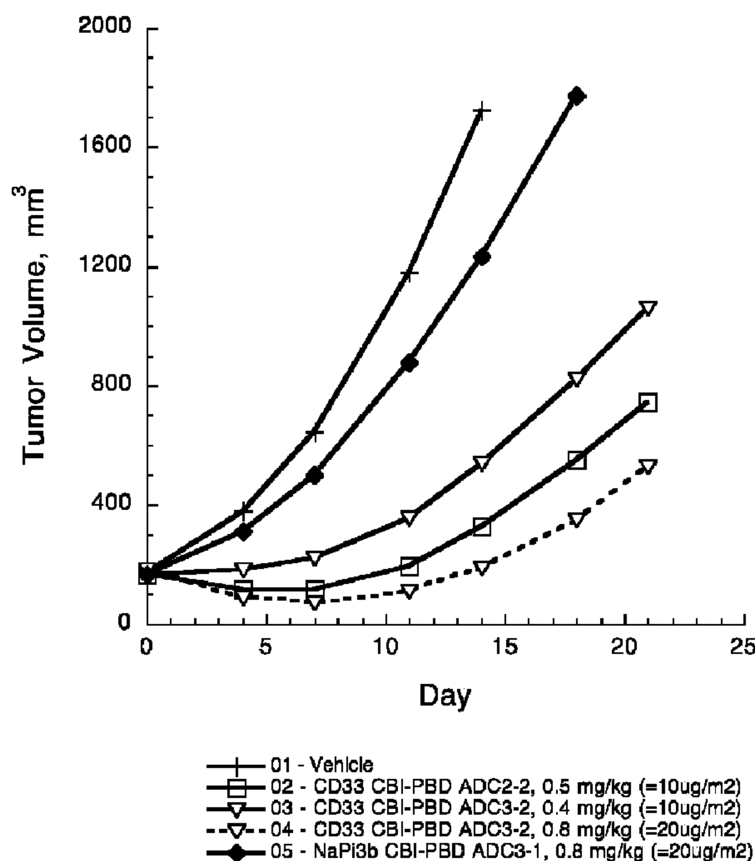
Figure 1 (HL-60)
