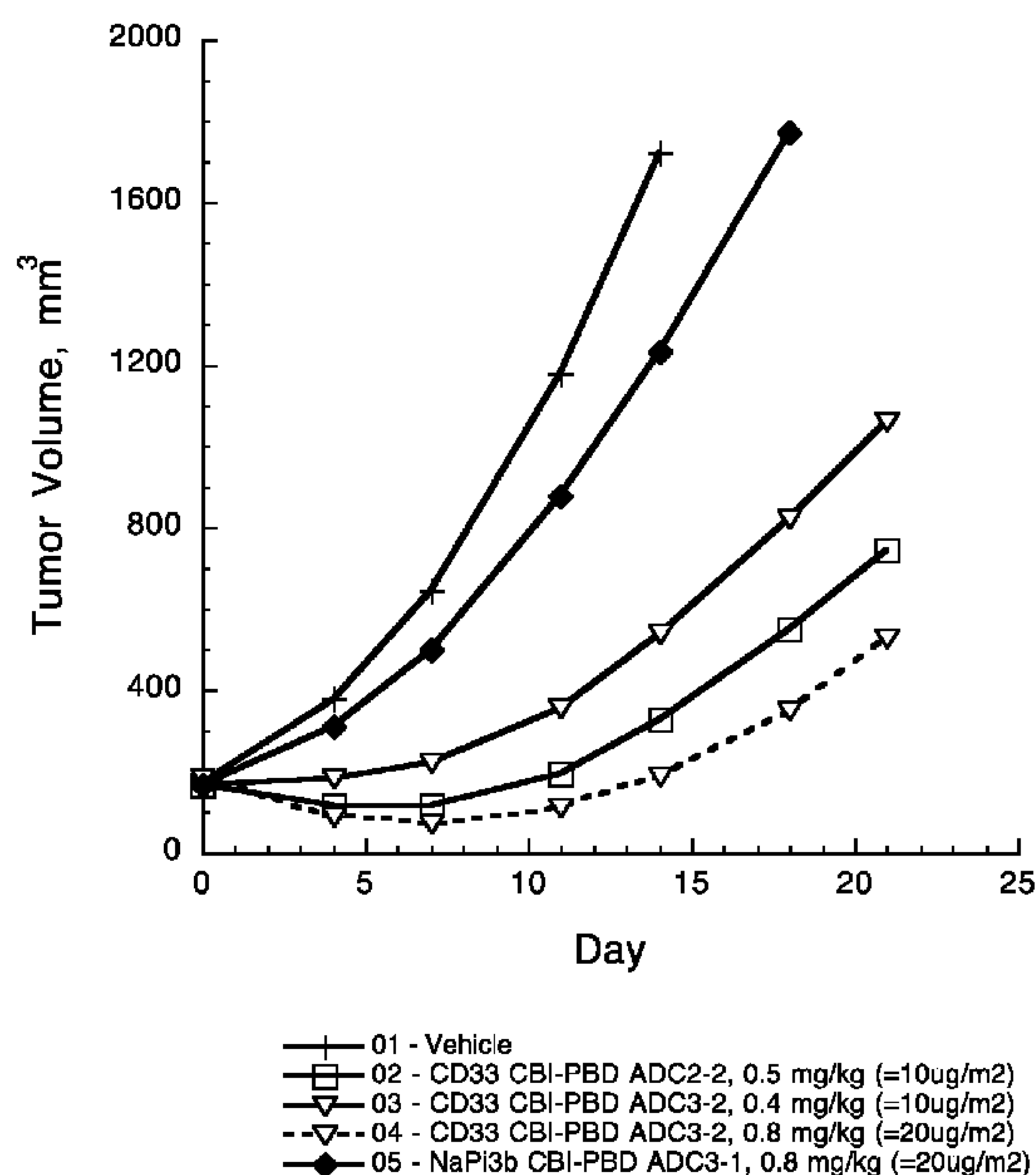
Figure 1 (HL-60)
