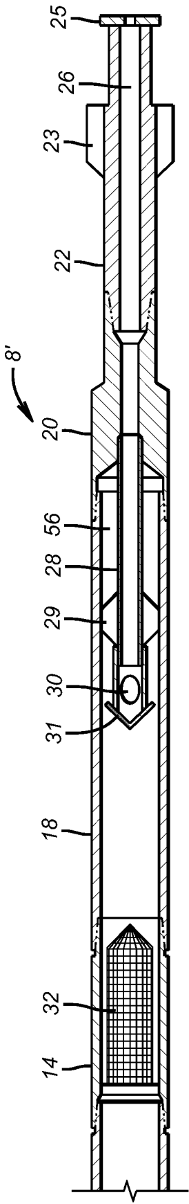
(PRIOR ART) FIG. 4
