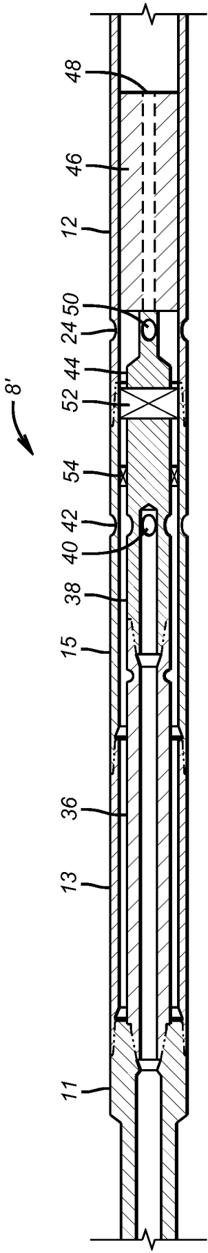
(PRIOR ART) FIG. 3
