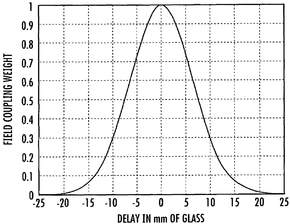
IMPULSE RESPONSE OF 10 GHz BANDPASS GAUSSIAN FILTER
