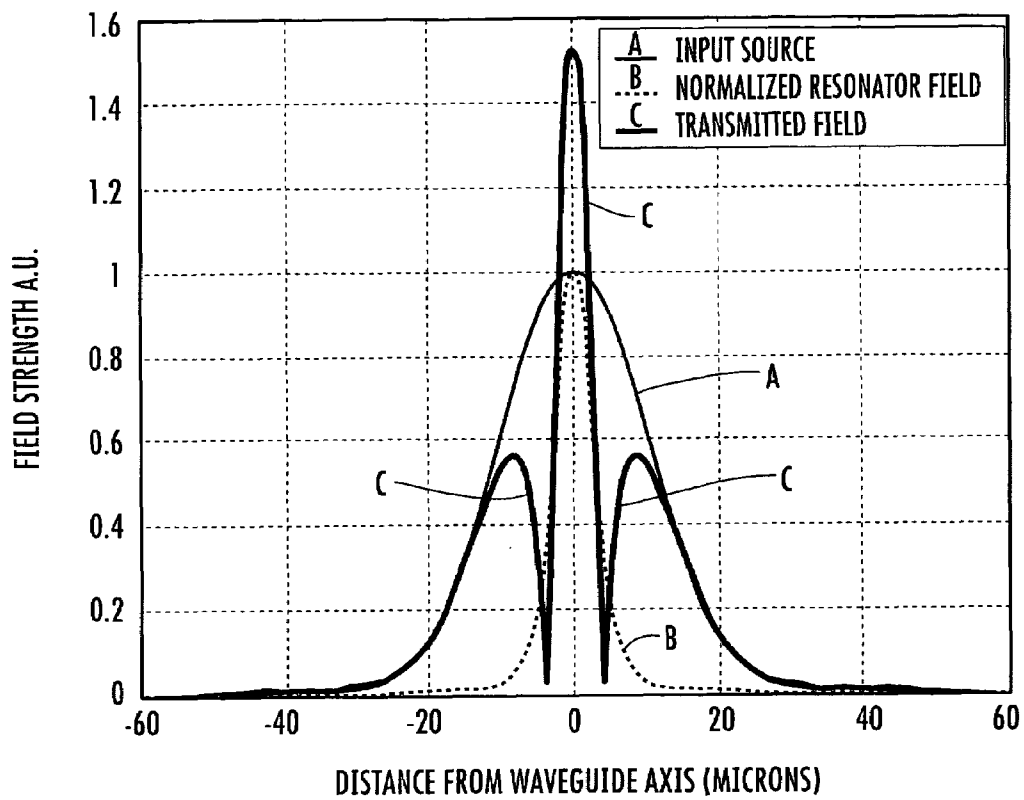
STEADY STATE FIELD PATTERNS
