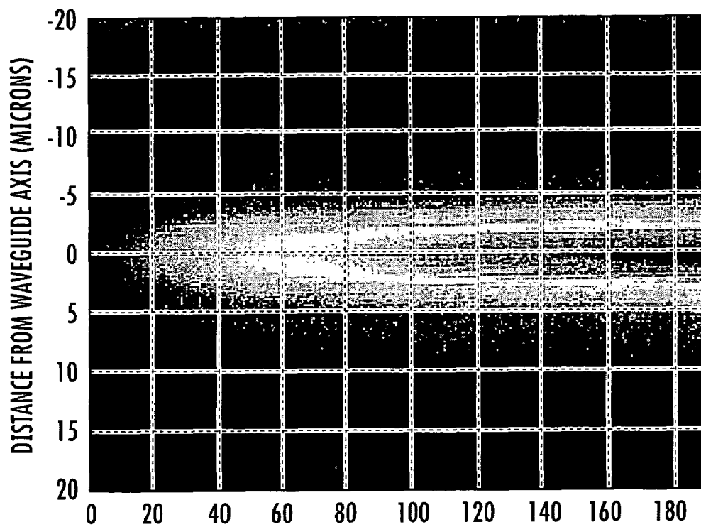
TIME IN PICOSECONDS TRANSIENT FIELD PATTERNS IN RESONATOR GUIDE
