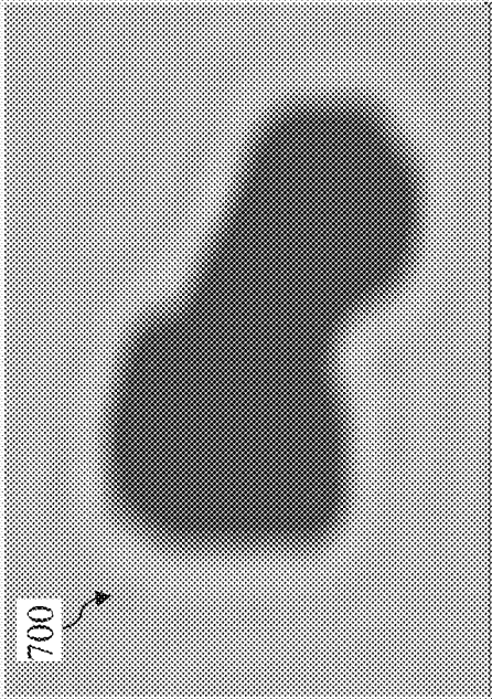
Aerial Image on wafer
