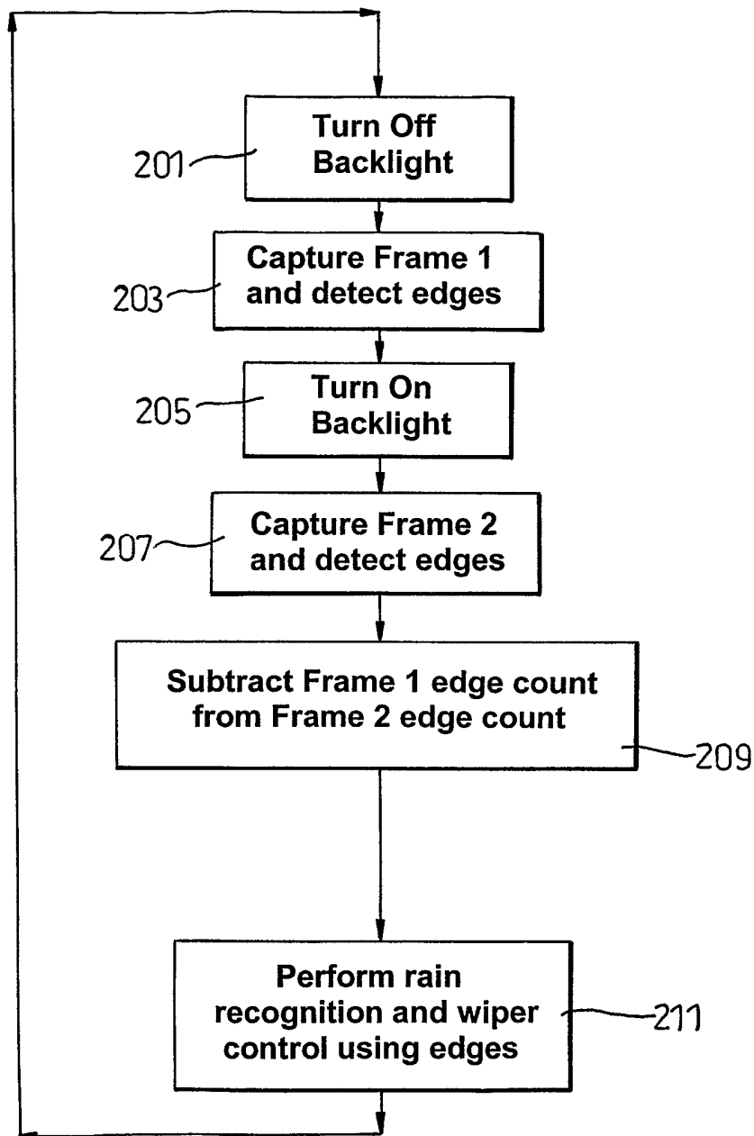
Edge Count Subtraction Control Diagram
