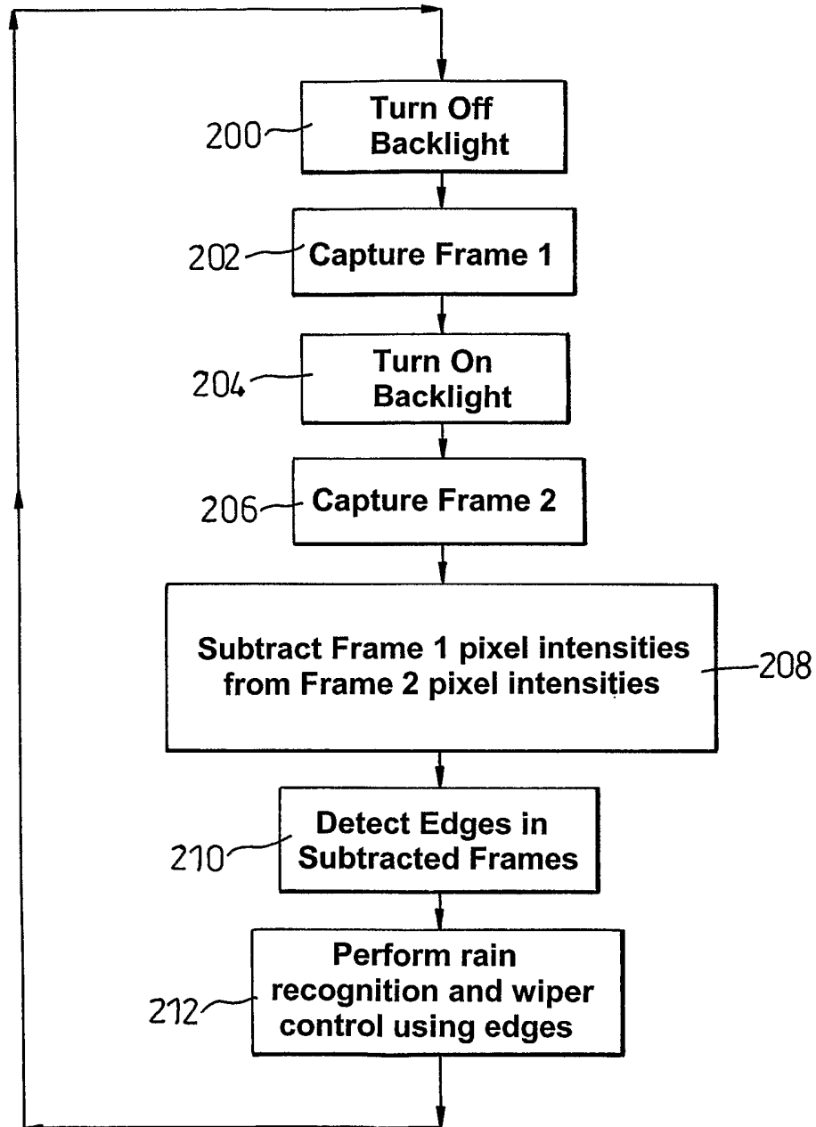
Frame Subtraction Control Diagram
