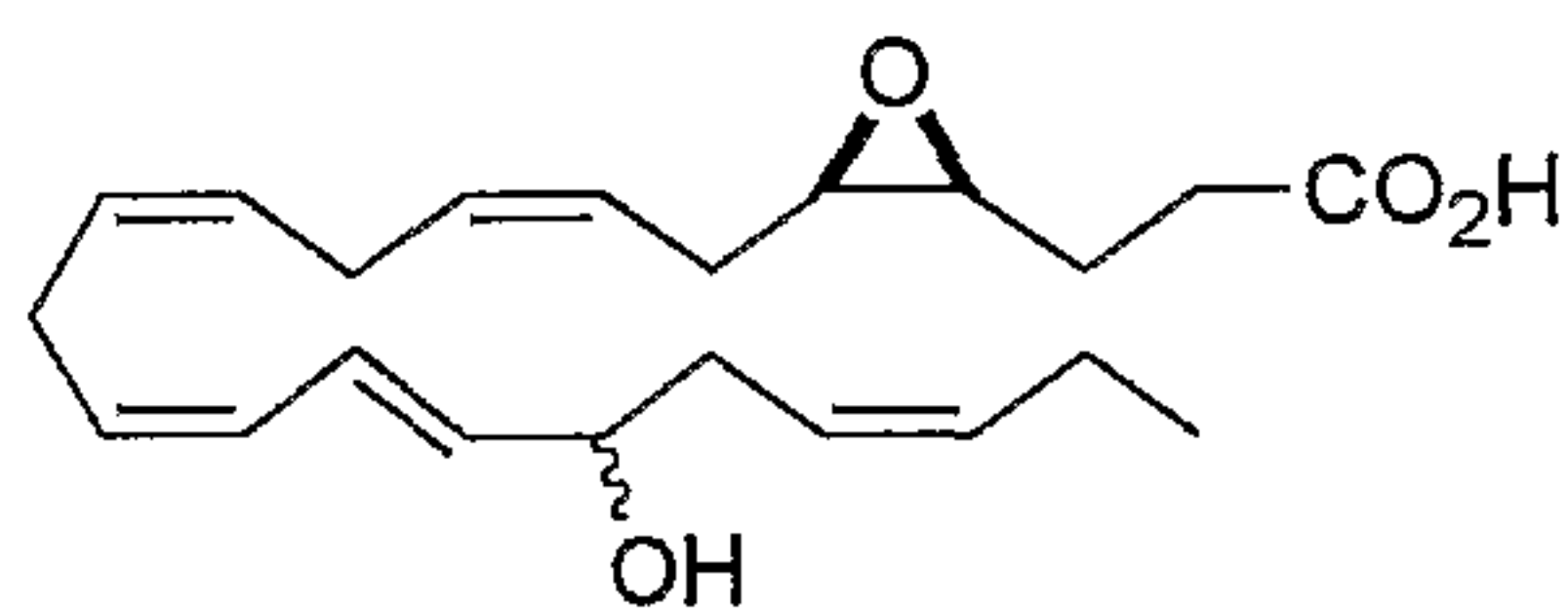
4,5-Epoxy-17-OH DPA
