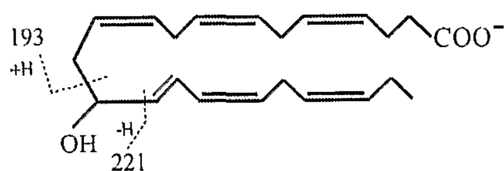
13-hydroxy DHA
