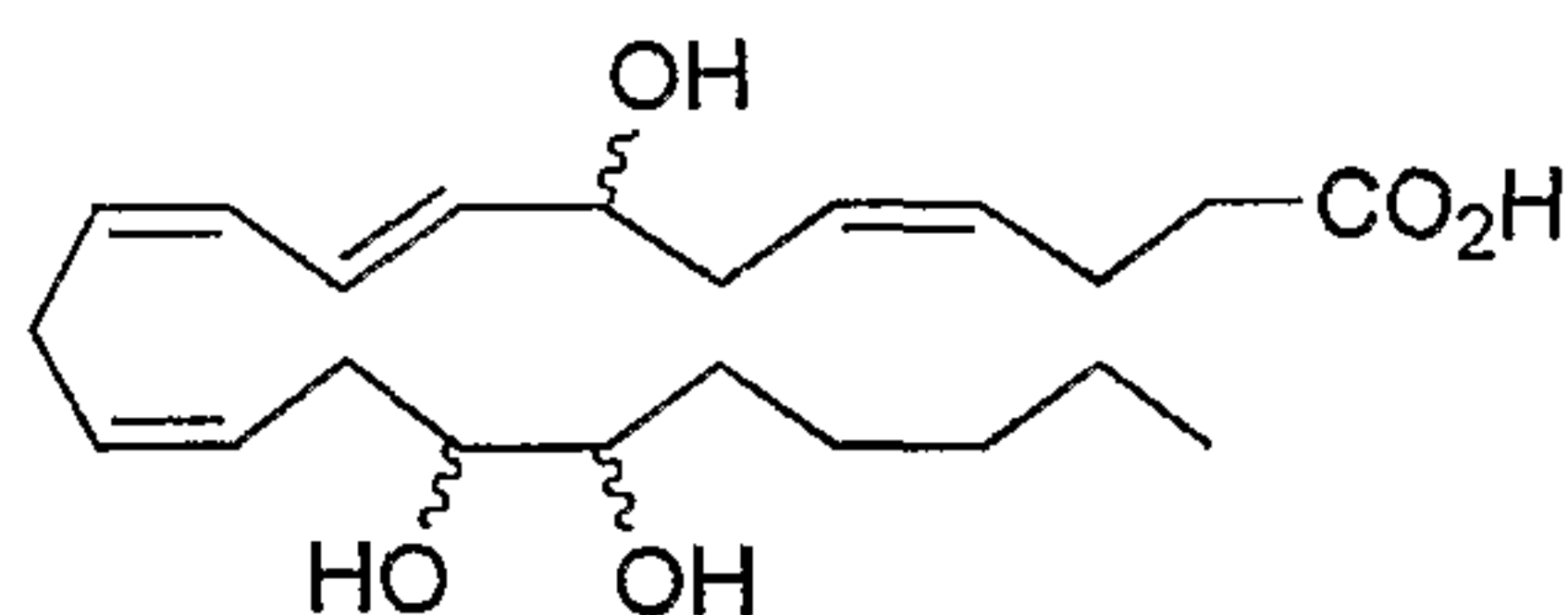
7,16,17-Trihydroxy DTAn-6
