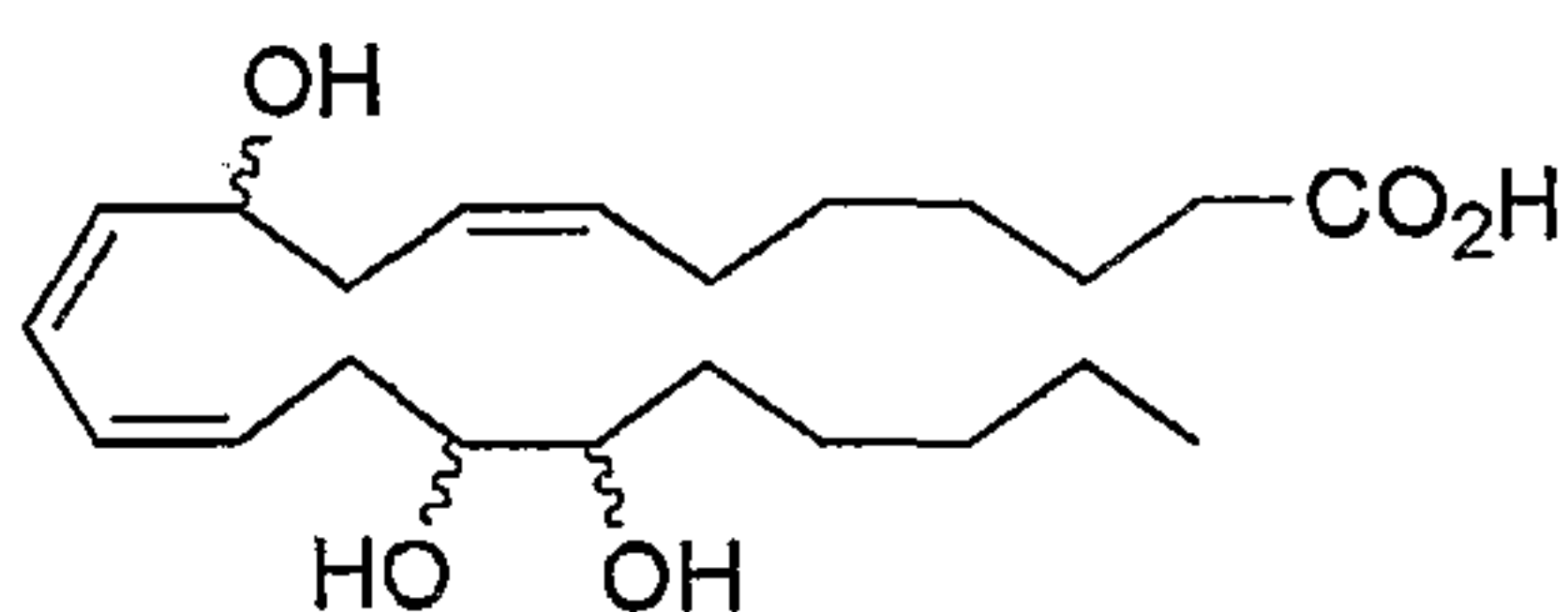
10,16,17-Trihydroxy DTRAn-6
