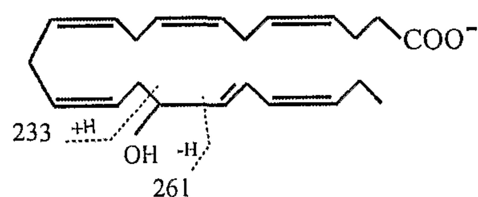
16-hydroxy DHA
