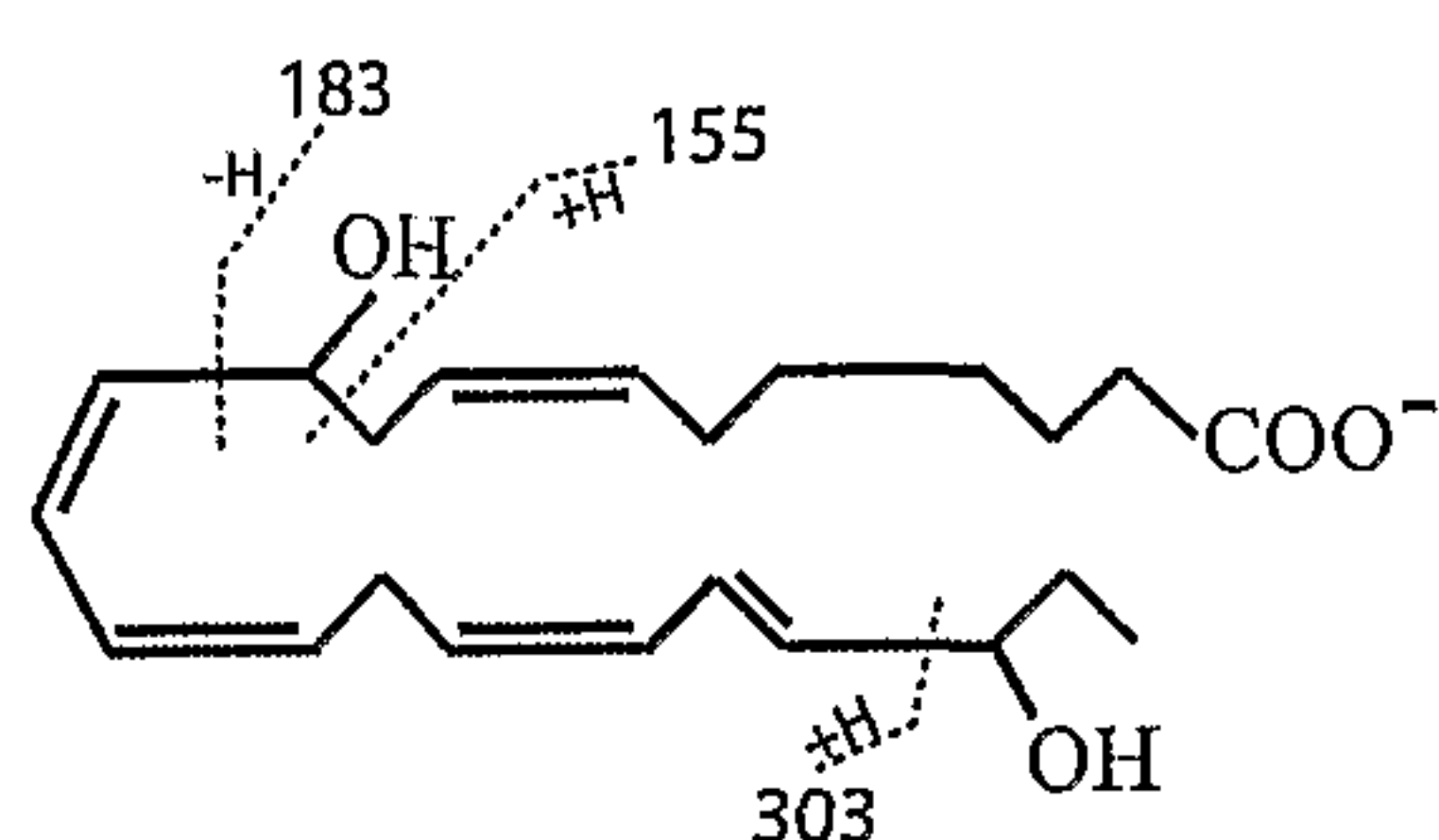
10,20 dihydroxy DPAn-3
