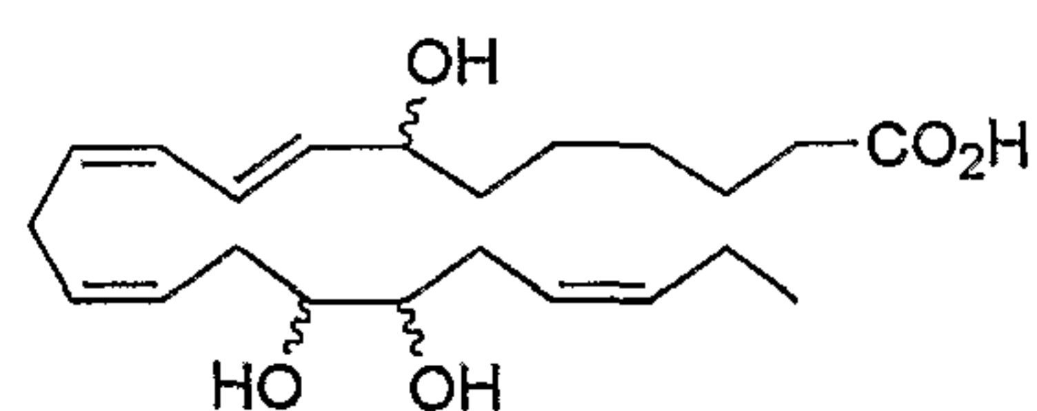
7,16,17-Trihydroxy DTAn-3
