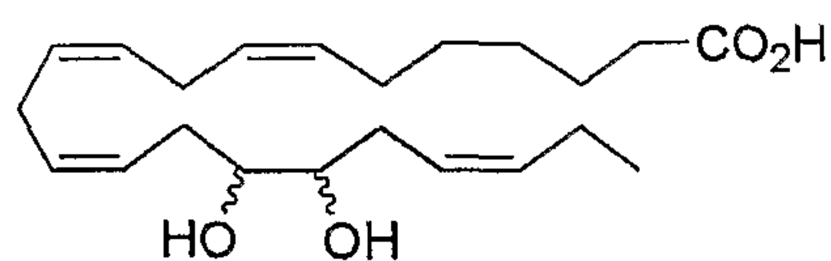
16,17-Dihydroxy DTAn-3
