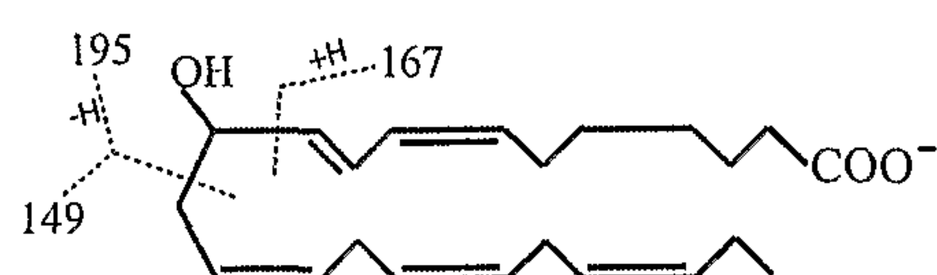
11-hydroxy DPAn-3
