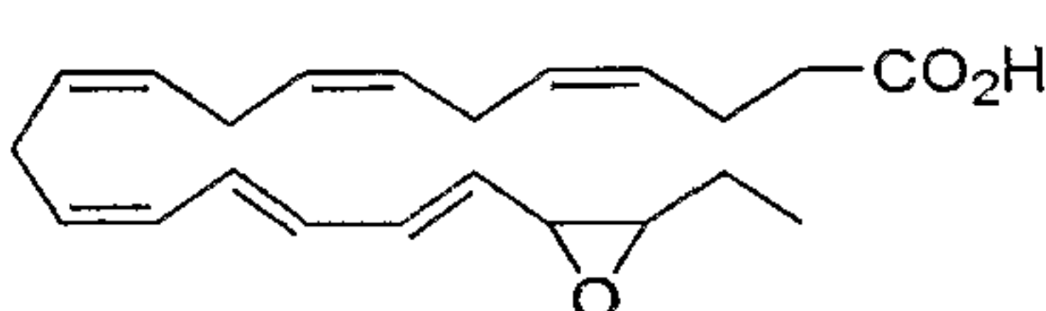
19,20-Epoxy-DHA
