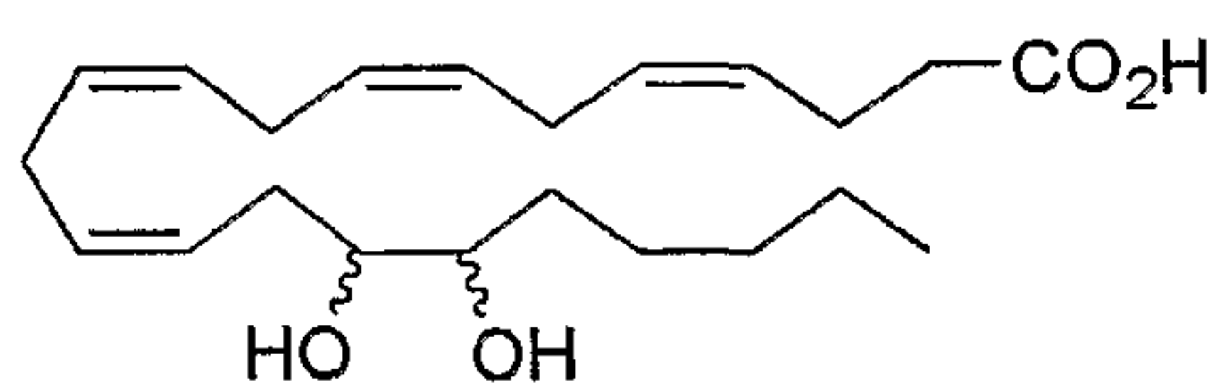
16,17-Dihydroxy DTAn-6
