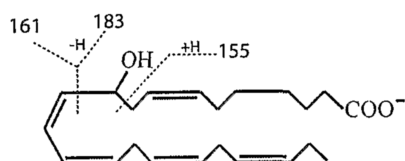
10-hydroxy DPAn-3
