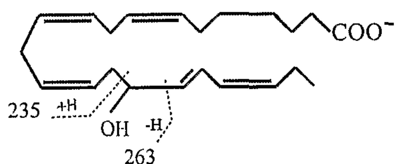
16-hydroxy DPAn-3
