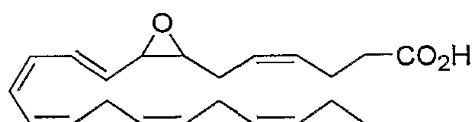
7,8-Epoxy DHA
