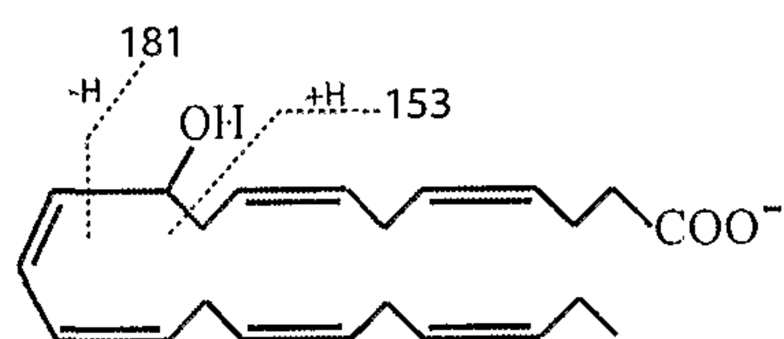
10-hydroxy DHA
