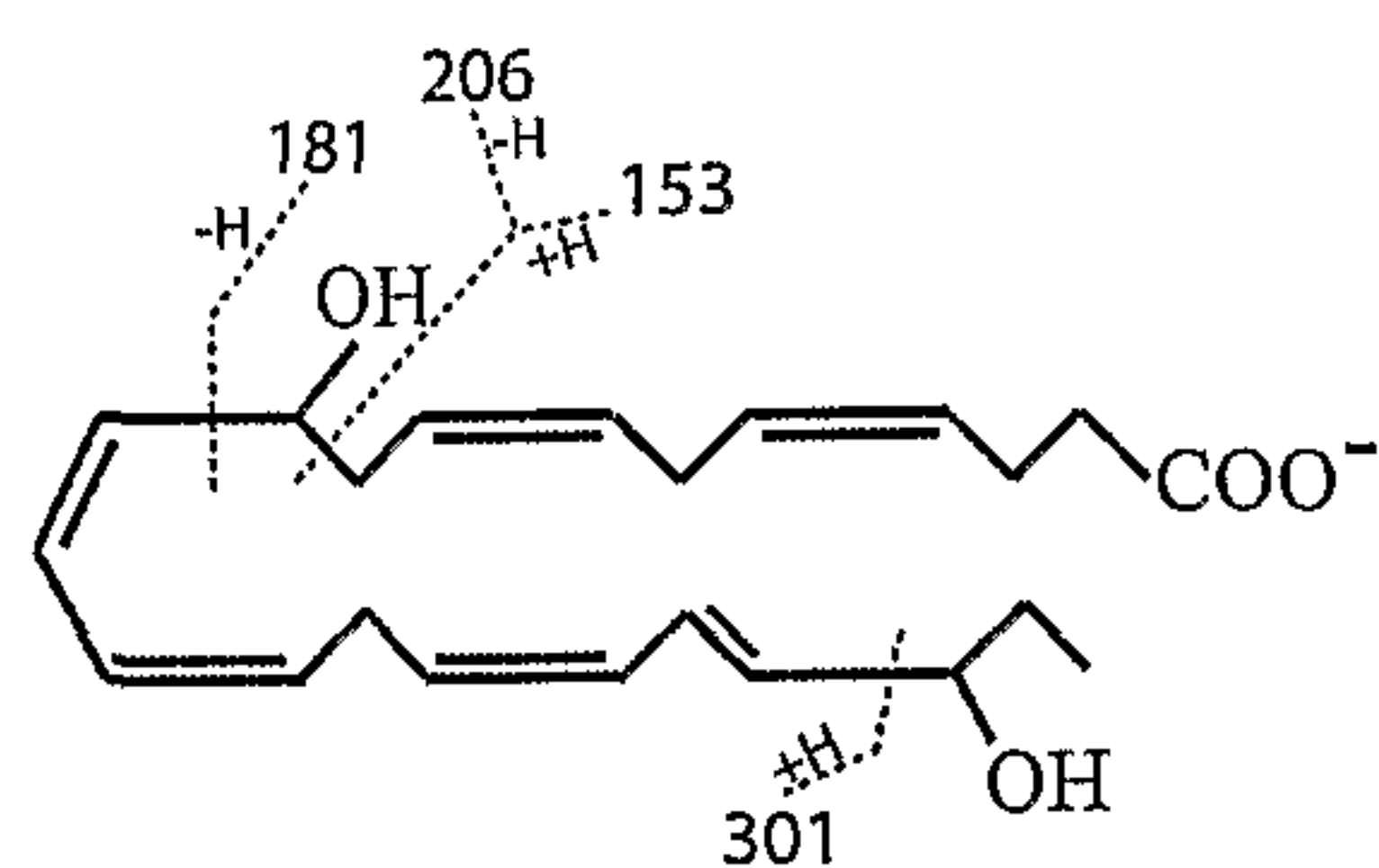
10,20- dihydroxy DHA
