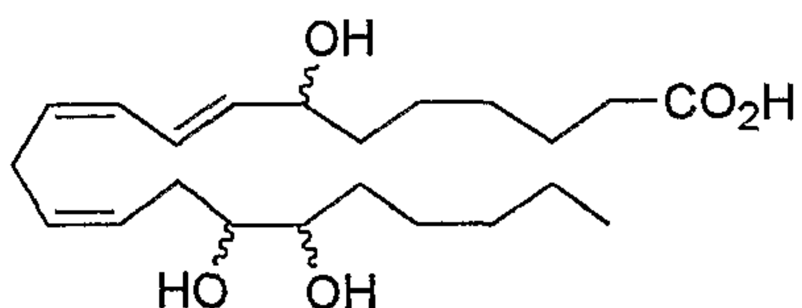
7,16,17-Trihydroxy DTRAn-6
