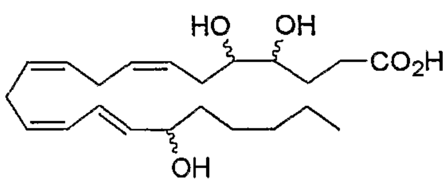
4,5,17-Trihydroxy DTAn-6
