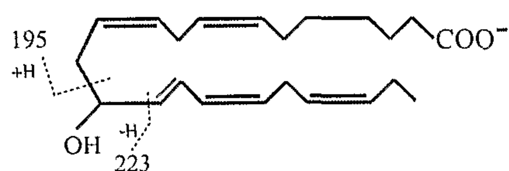
13-hydroxy DPAn-3
