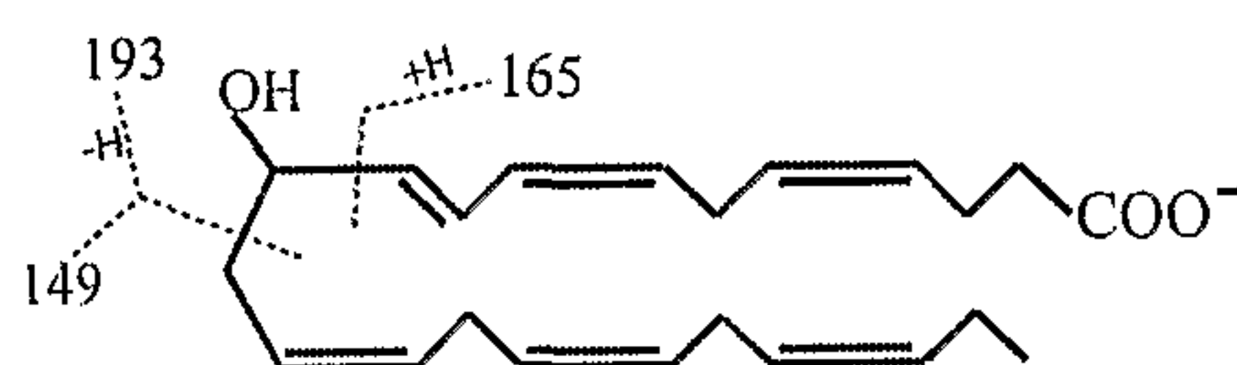
11-hydroxy DHA
