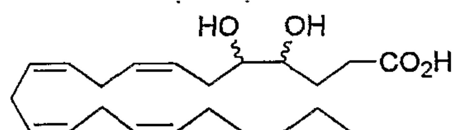
4,5-Dihydroxy DTAn-6
