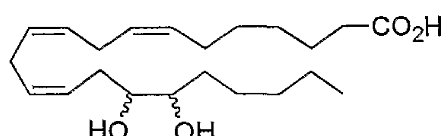
16,17-Dihydroxy DTRAn-6
