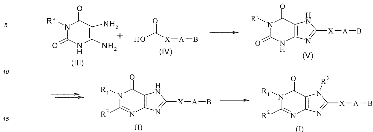
Scheme 1:
