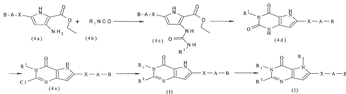
Scheme 6:
