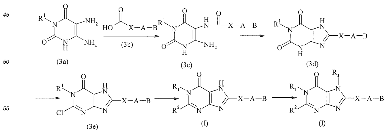
Scheme 5:
