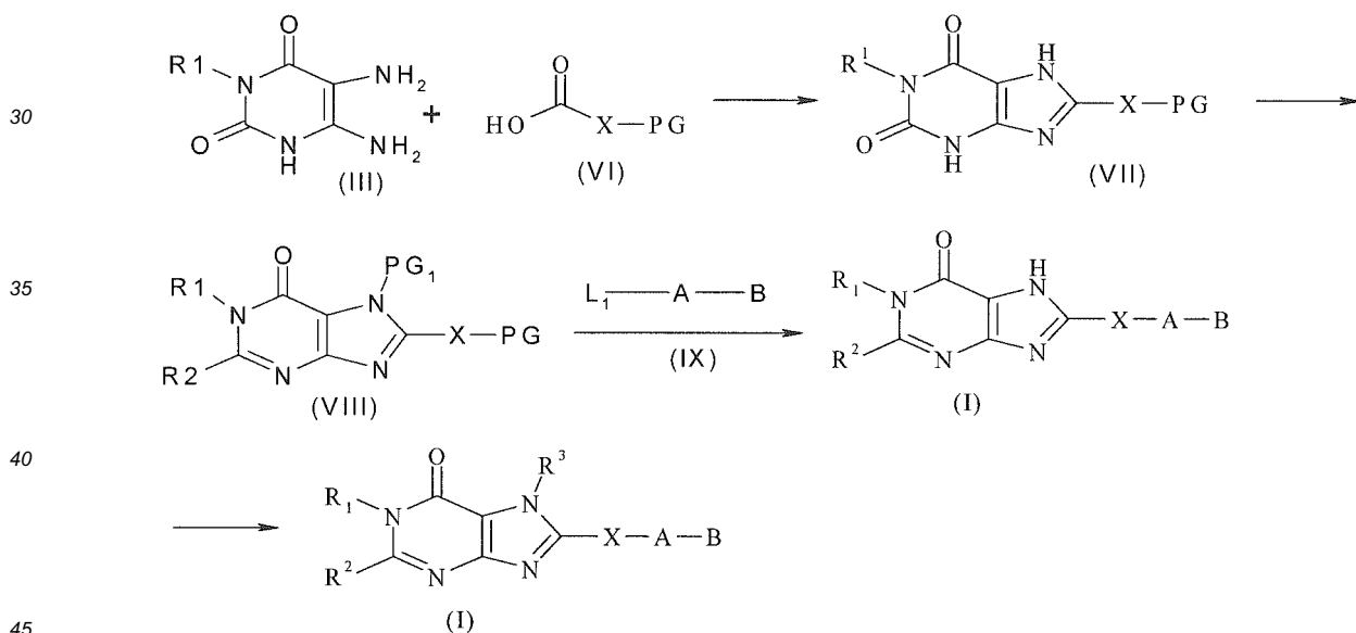
Scheme 2:
