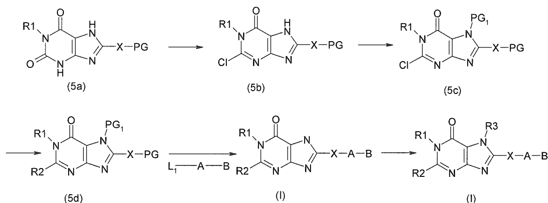
Scheme 7:
