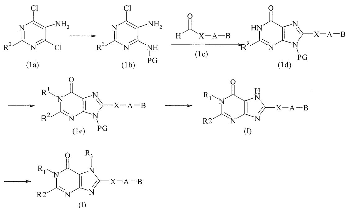
Scheme 3:
