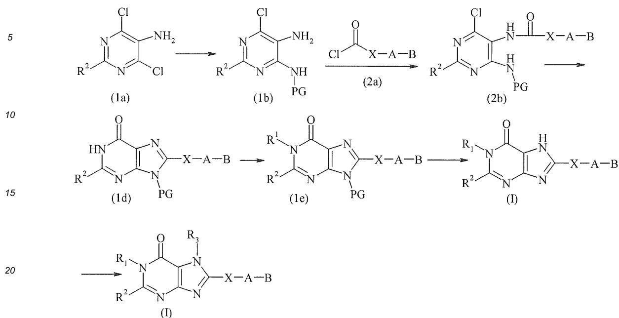
Scheme 4:
