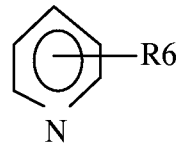
Formula C – aromatic tertiary amine
