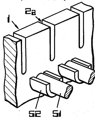
FIG. 5 PRIOR ART
