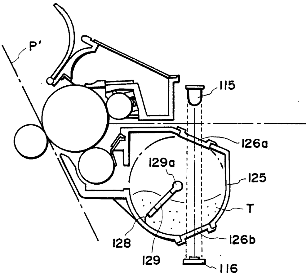
FIG. 21 PRIOR ART
