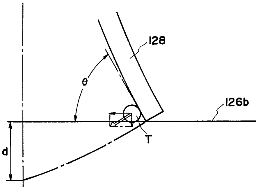
FIG. 23(b) PRIOR ART
