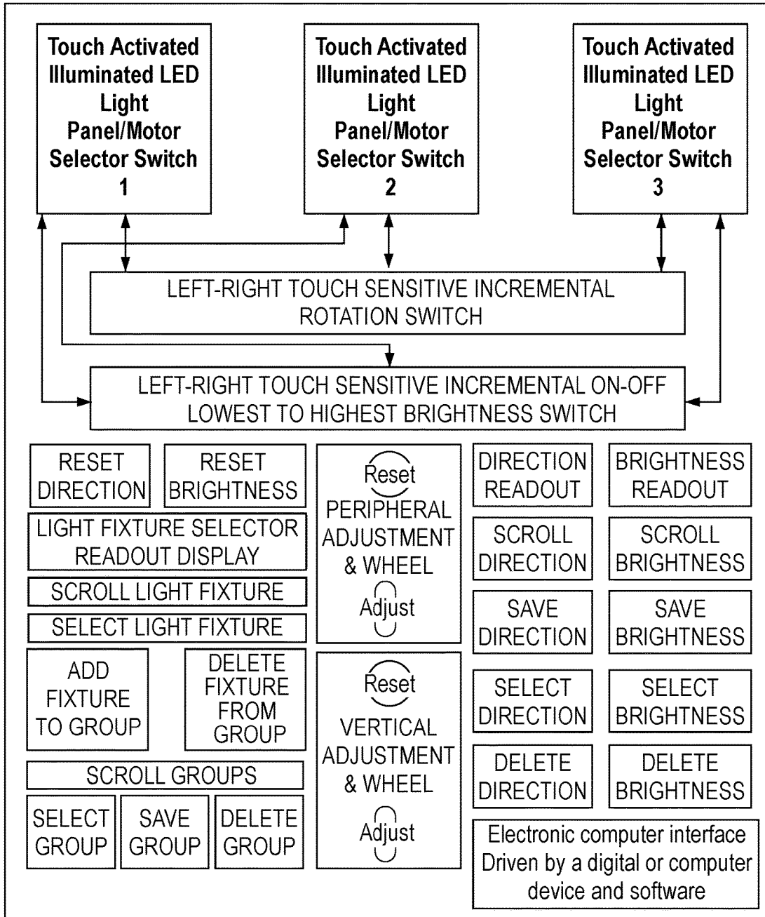
CONTROLLER INTERFACE BLOCK DIAGRAM WITH COMPUTER INTERFACE
