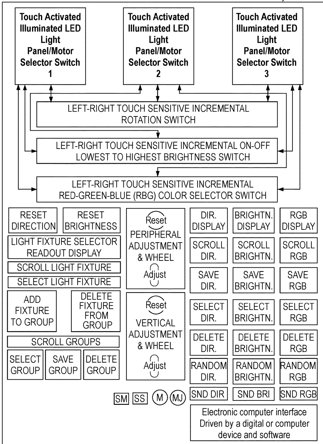
Fig. 18 RGB-SOUND CONTROLLER BLOCK DIAGRAM 1800 w/ COMPUTER INTERFACE
