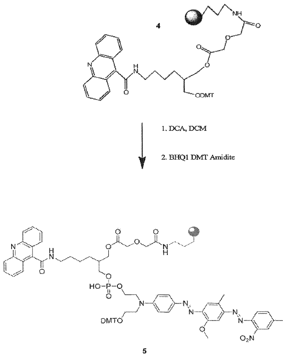
Scheme 2
