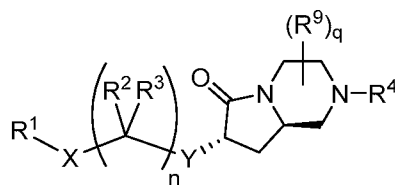
Formula (Id);
