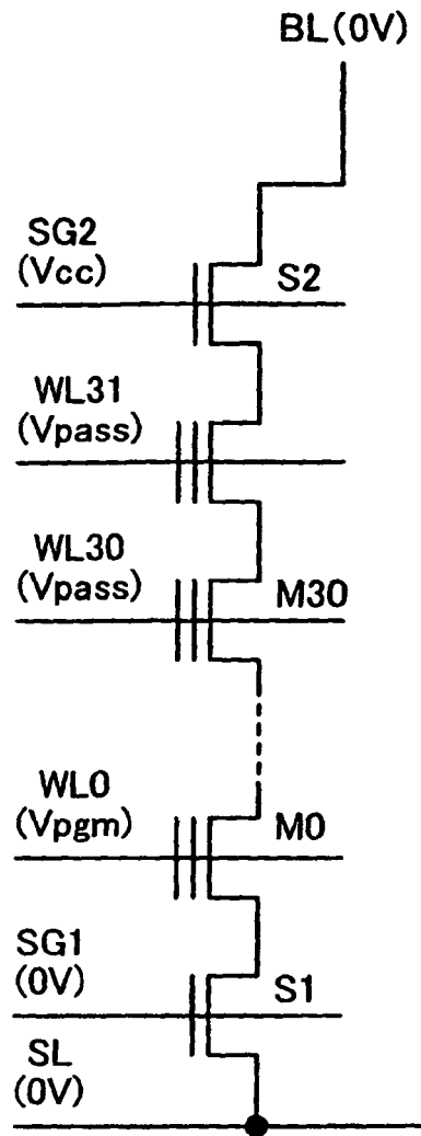
FIG. 19A "0" writing
