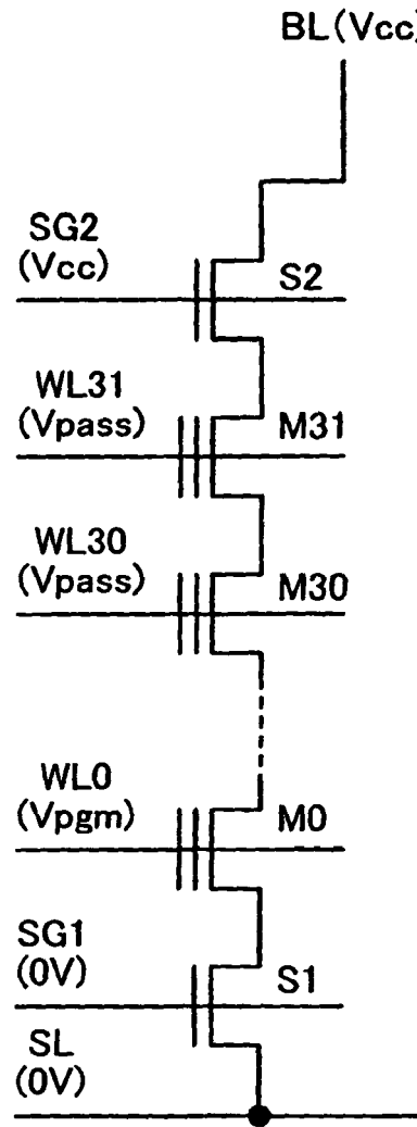
FIG. 19B "1" writing
