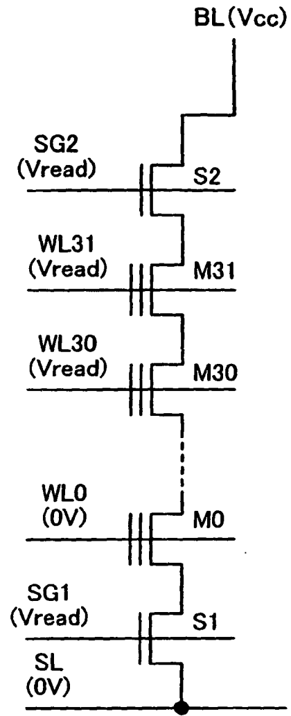
FIG. 20B reading
