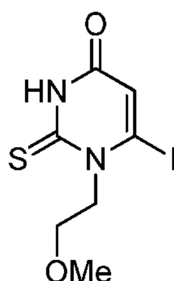
6-Iodo-1-(2-methoxyethyl)-2-thioxo-2,3-dihydropyrimidin-4(1H)-one
