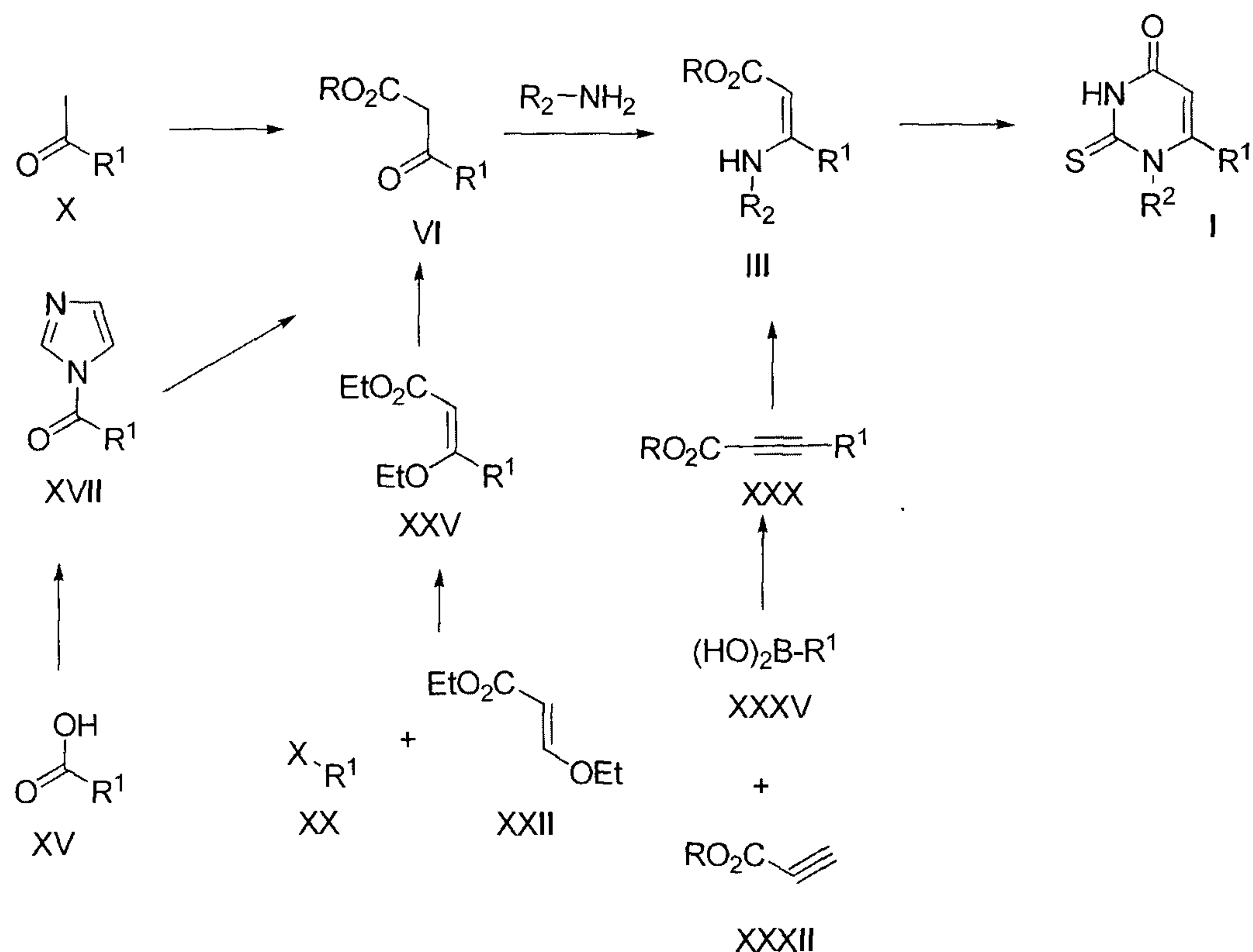
SCHEME I
