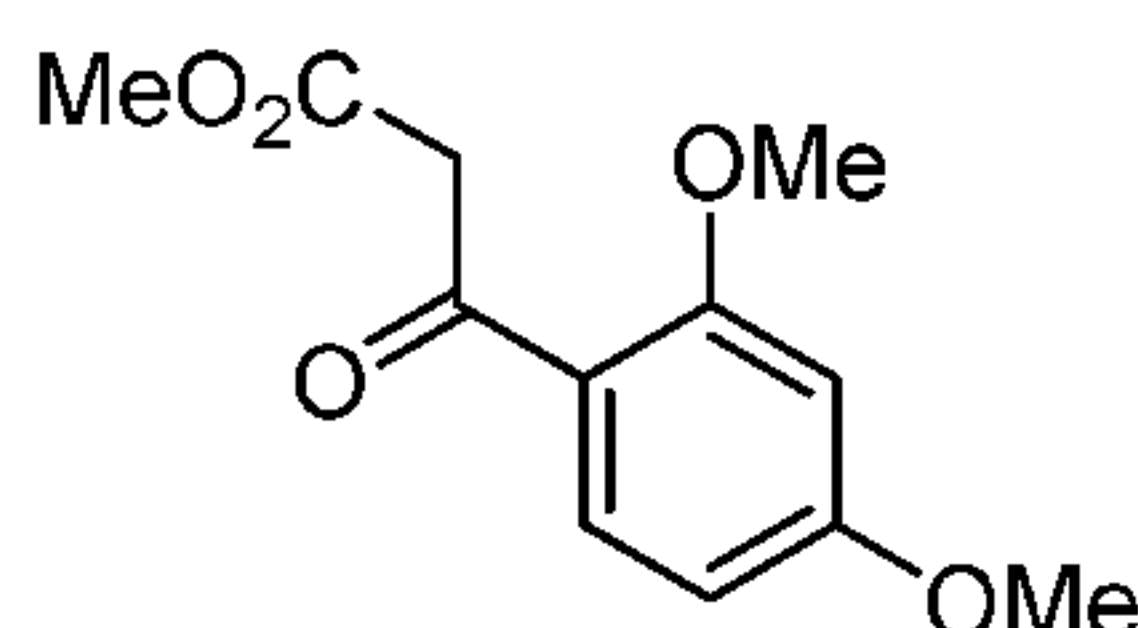
Methyl 3-(2,4-dimethoxyphenyl)-3-oxopropanoate
