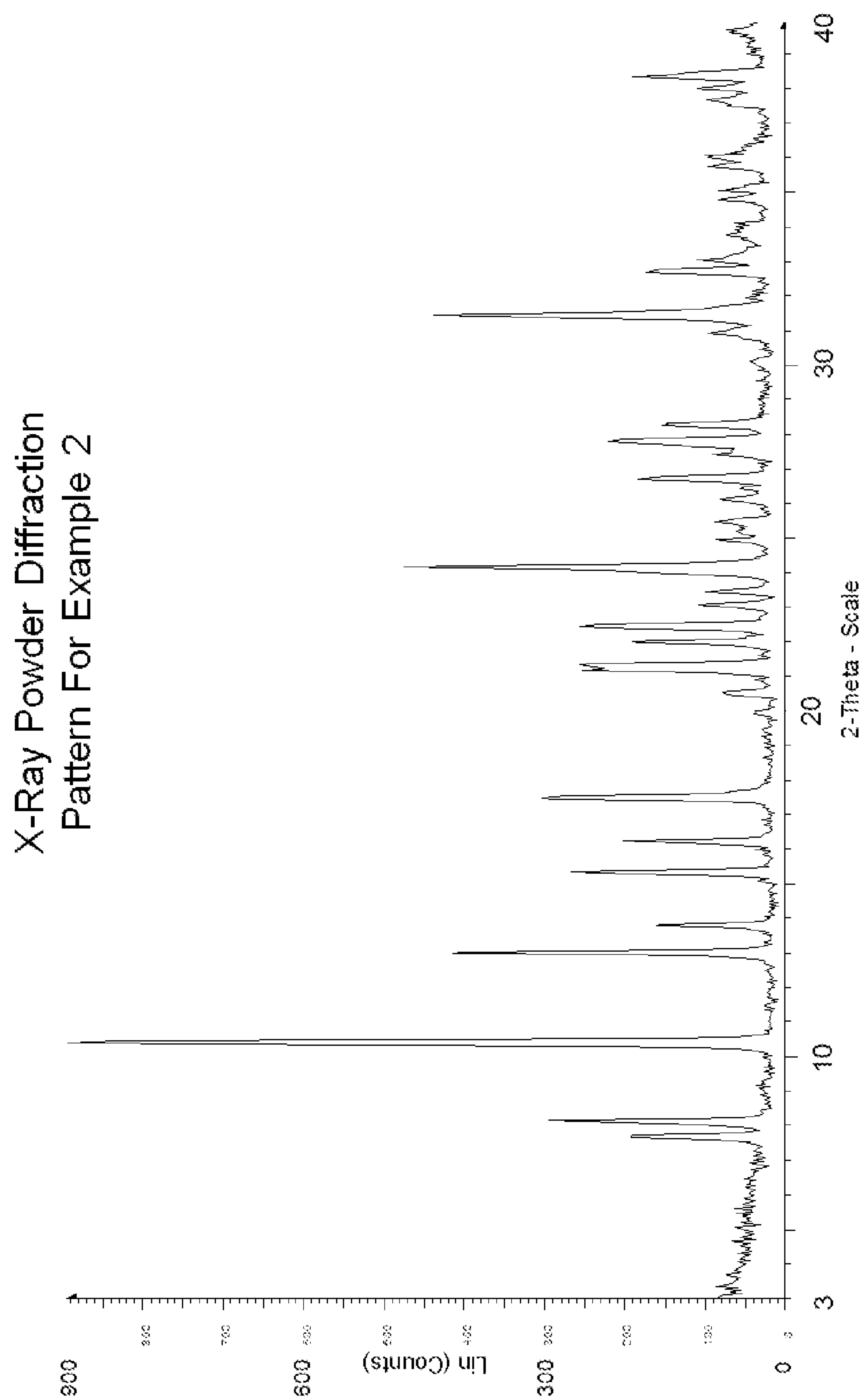
FIG. 2. X-ray powder diffraction pattern of Example 2.
