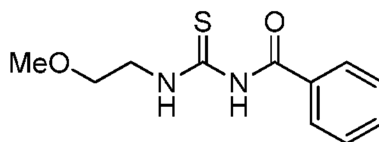
N-((2-Methoxyethyl)carbamothioyl)benzamide
