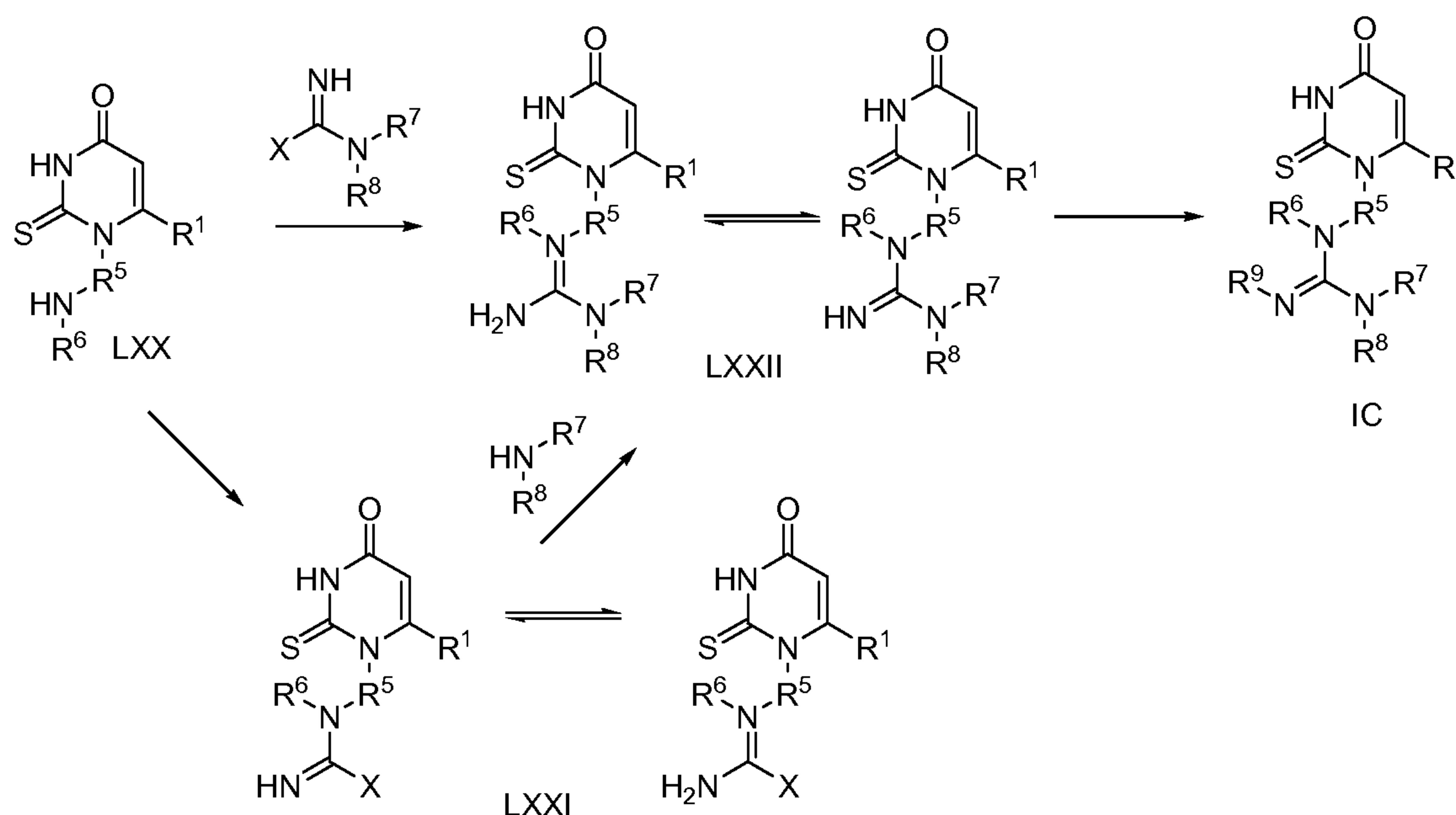
SCHEME IV
