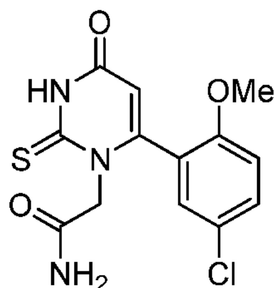
2-(6-(5-Chloro-2-methoxyphenyl)-4-oxo-2-thioxo-3,4-dihydropyrimidin-1(2H)-yl)acetamide
