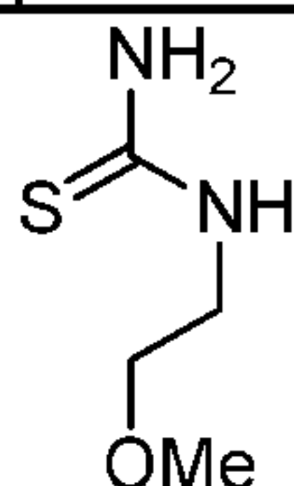
1-(2-Methoxyethyl)thiourea
