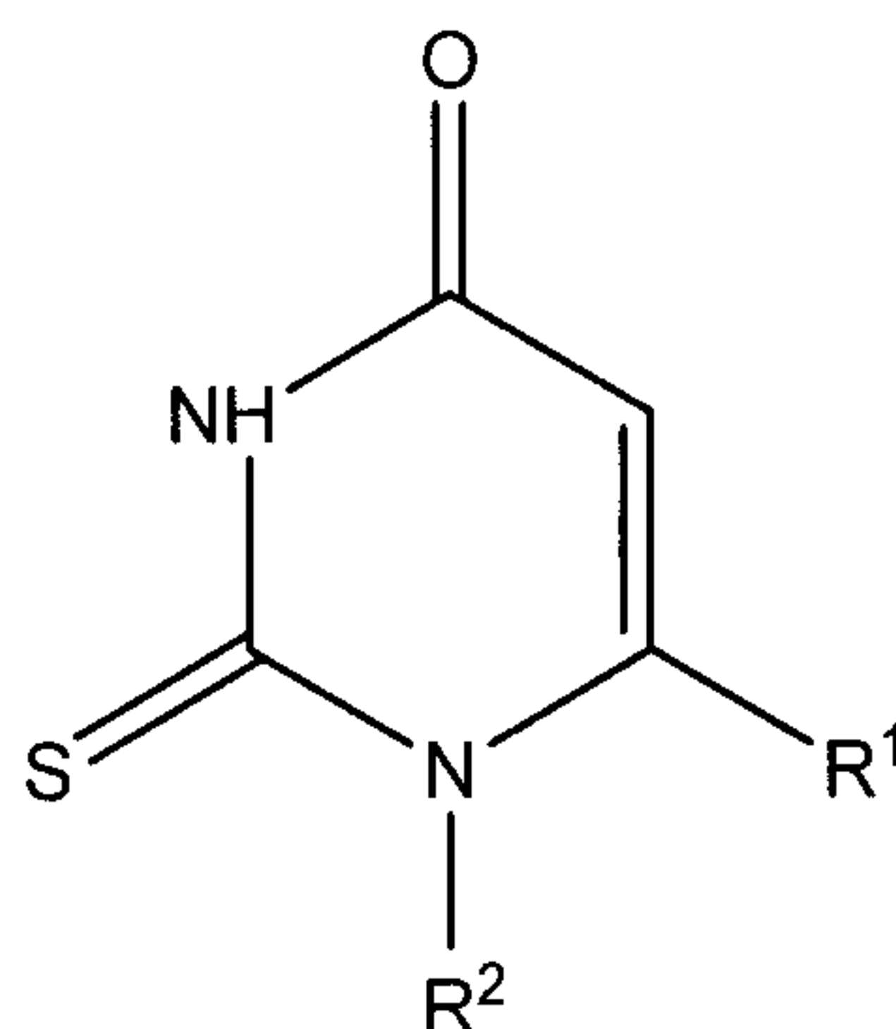
Formula I
