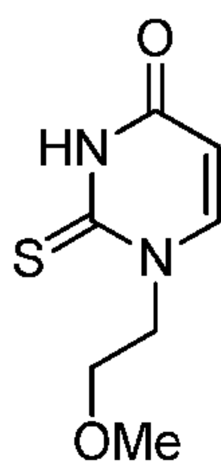
1-(2-Methoxyethyl)-2-thioxo-2,3-dihydropyrimidin-4(1H)-one
