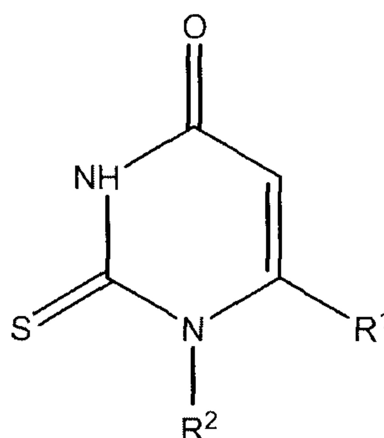
Formula I
