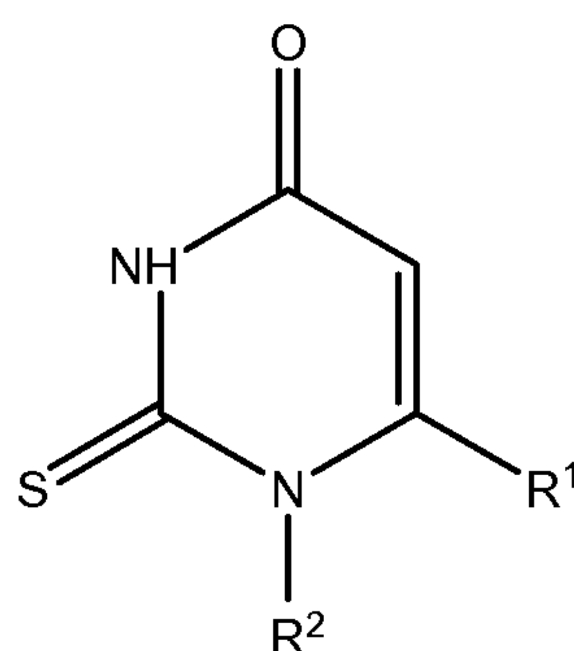
Formula IA
