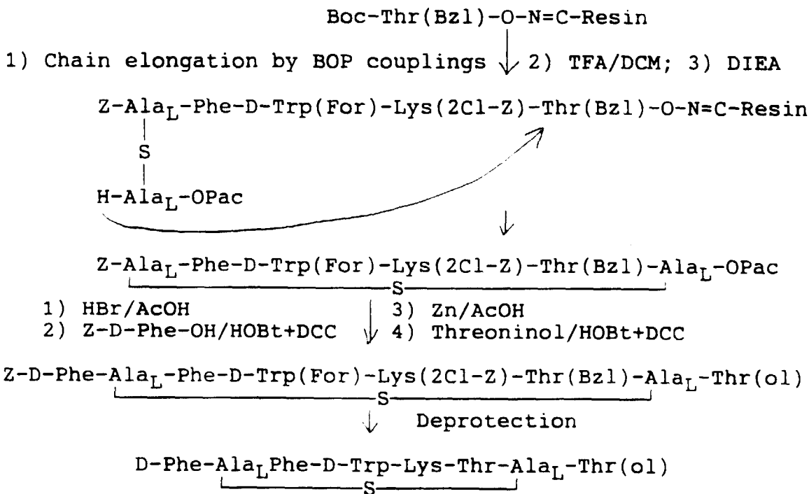
Scheme 2. Synthesis of Lanthionine-sandostatin Utilizing Cyclization on an Oxime Resin
