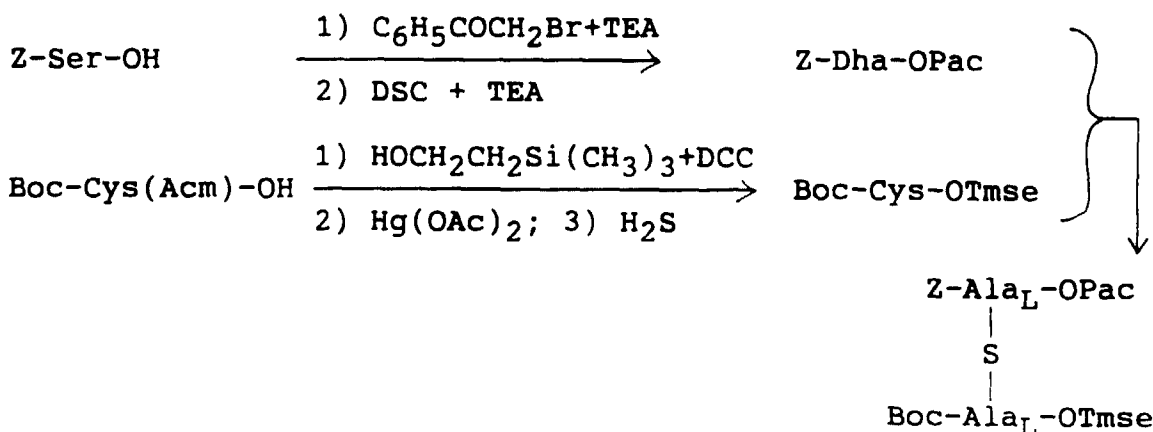
Scheme 1. Synthesis of Protected Lanthionine from Dehydroalanine
