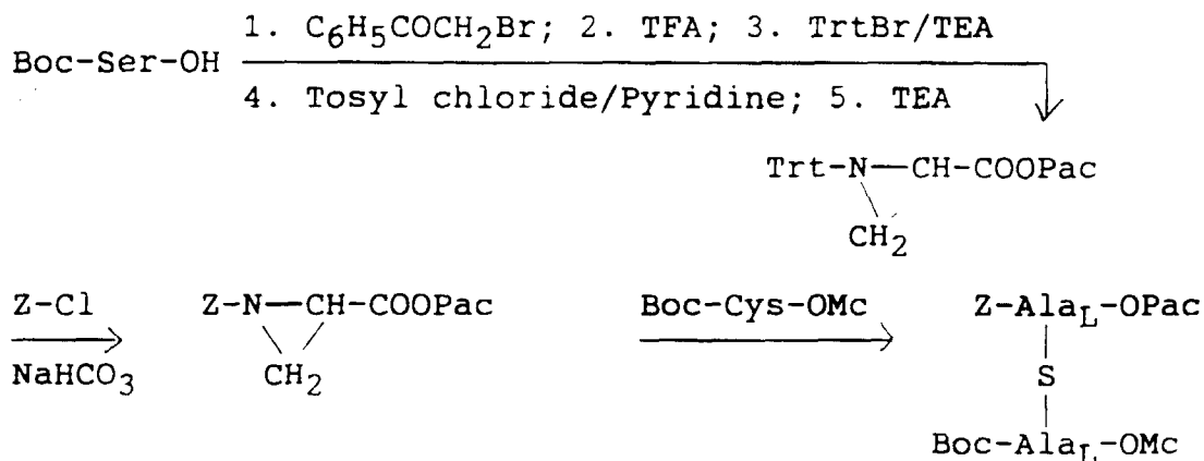
Scheme 4. Synthesis of Protected Lanthionine from Aziridine Derivatives
