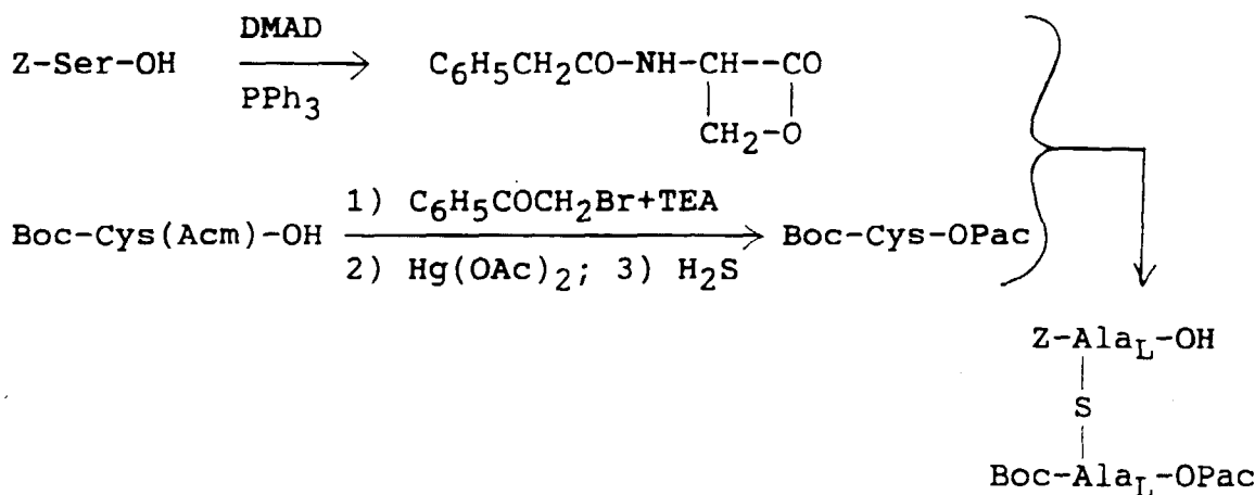
Scheme 3. Synthesis of Protected Lanthionine from Serine-lactone
