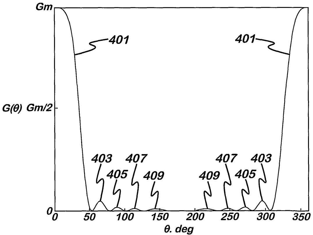
Fig. 4 Example of antenna gain
