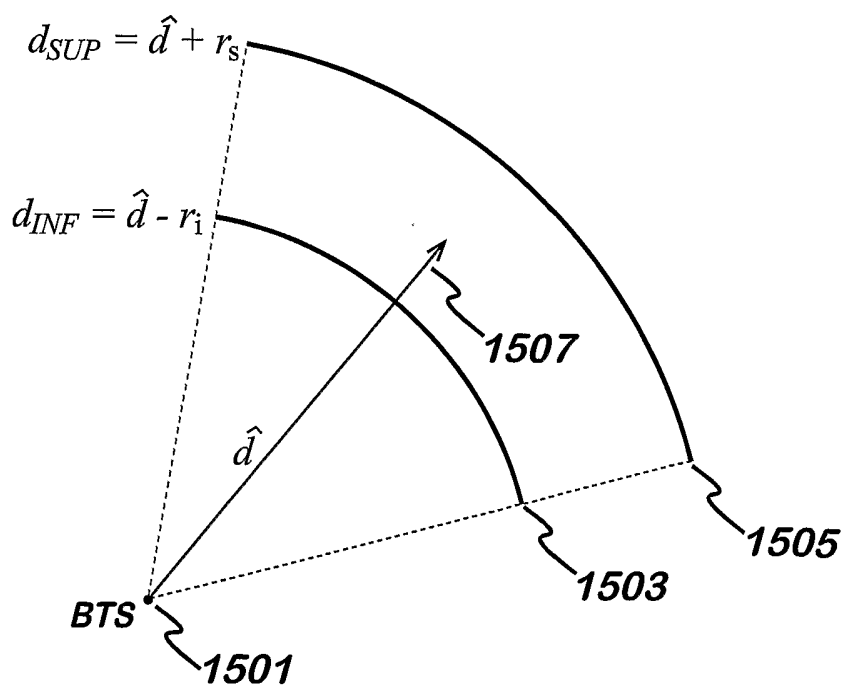
Fig. 15 Definition of estimate of distance and its confidence interval
