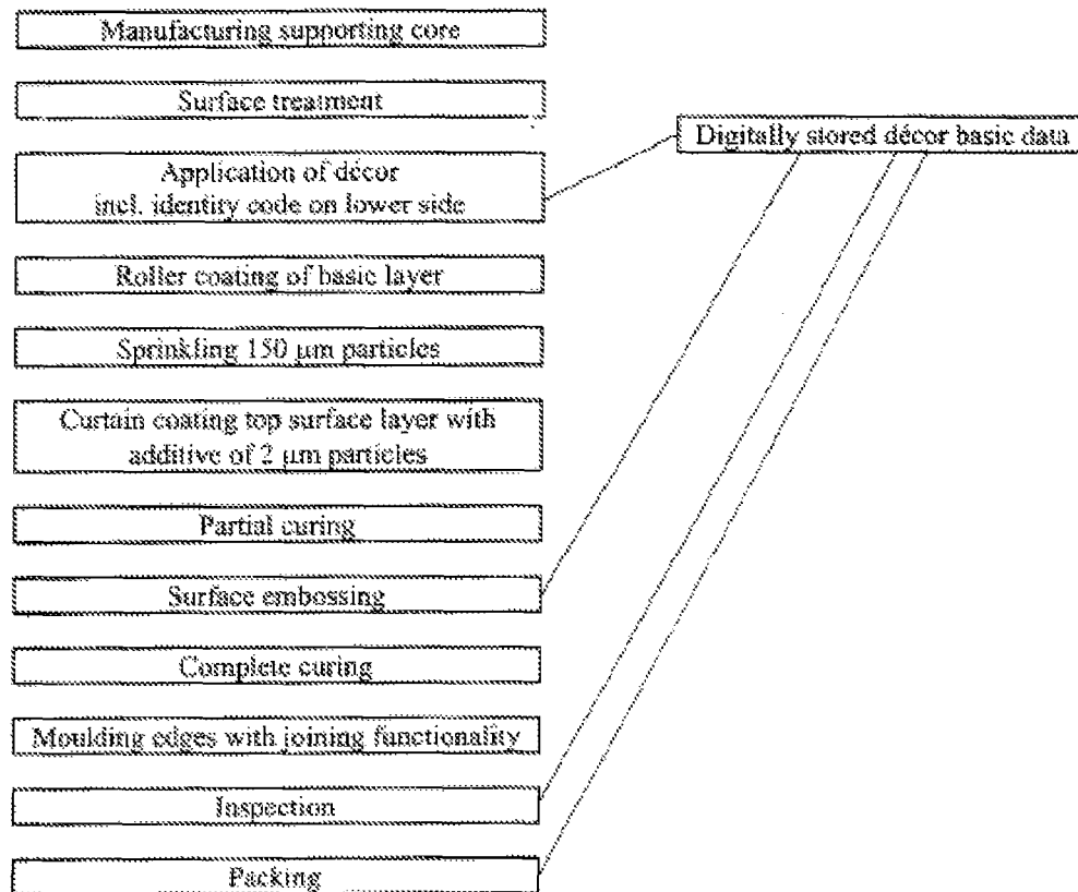
Process scheme 2
