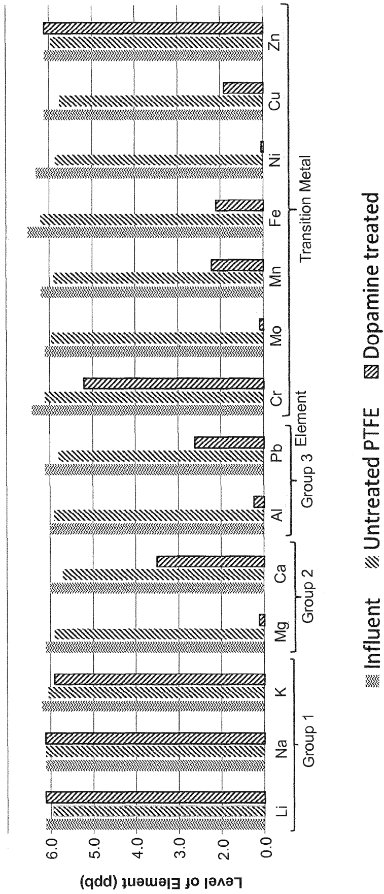
Figure 2 Metal Removal
