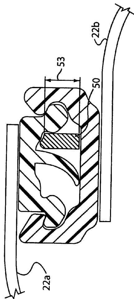
FIG. 10 (PRIOR ART)
