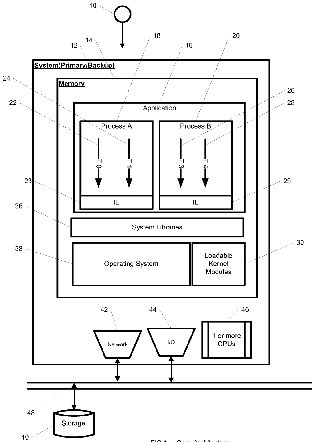
FIG.1 - Core Architecture
