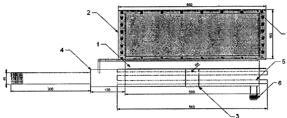
FRONT ELEVATION OF THE DESALINATION UNIT
