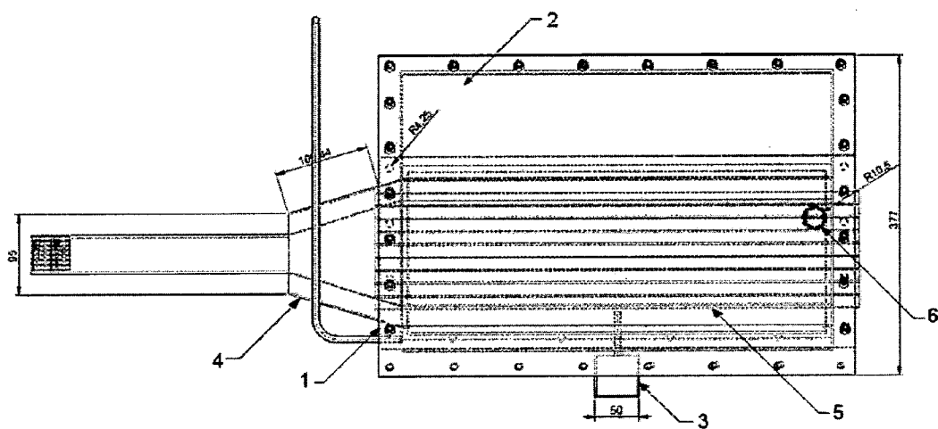
FIG. 2 TOP ELEVATION OF THE DESALINATION UNIT
