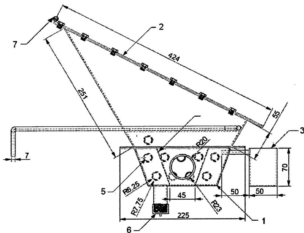
FIG. 3 SIDE ELEVATION OF THE DESALINATION UNIT
