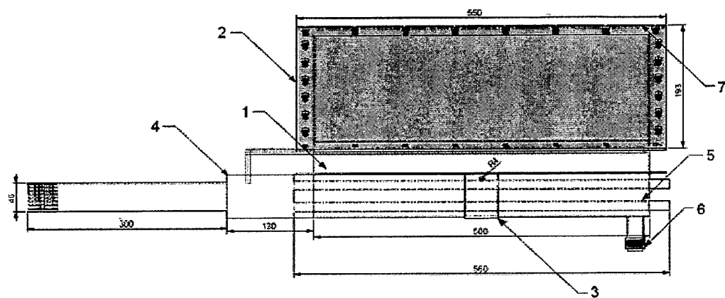
FIG. 1 FRONT ELEVATION OF THE DESALINATION UNIT
