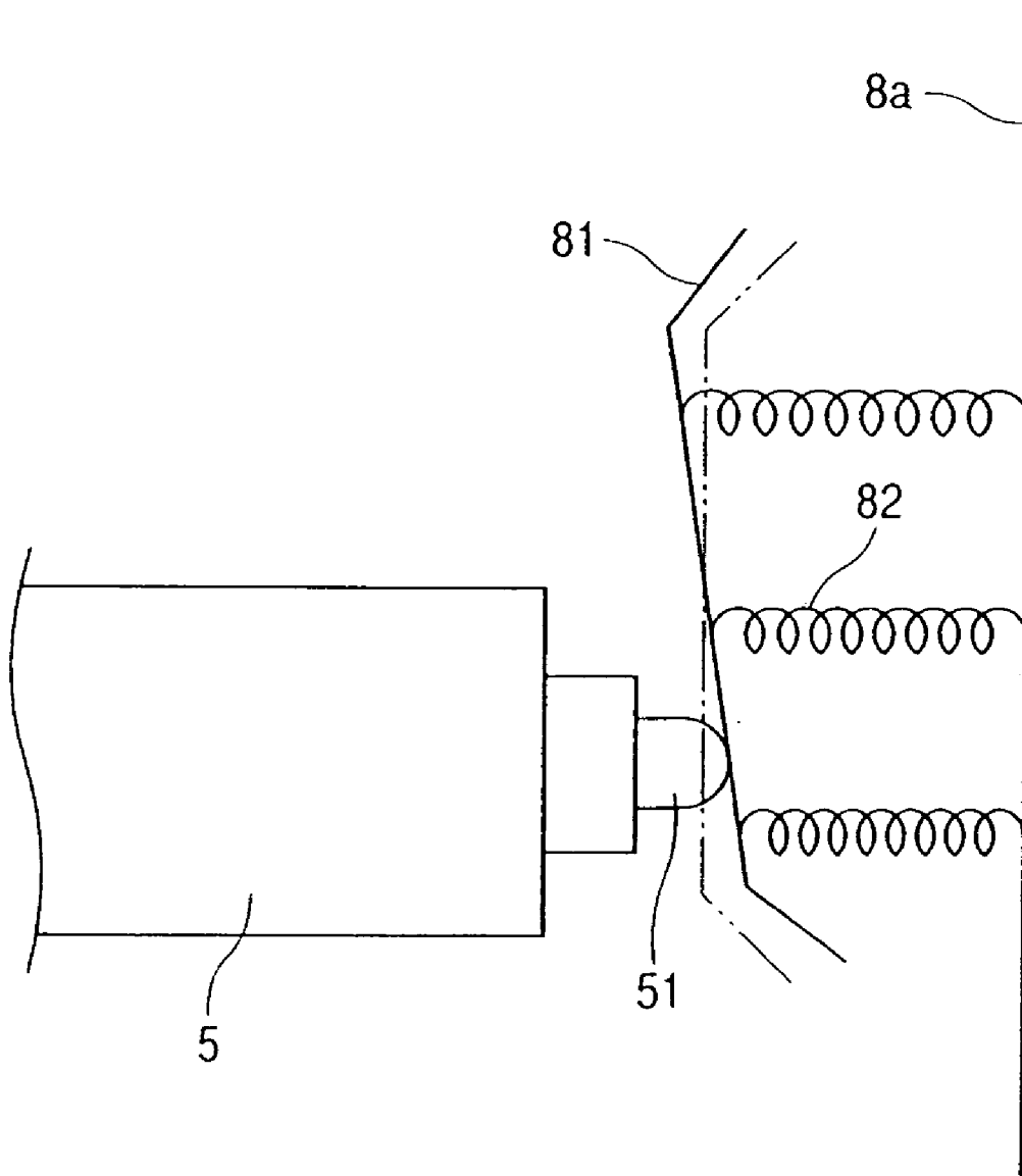
FIG. 14 PRIOR ART
