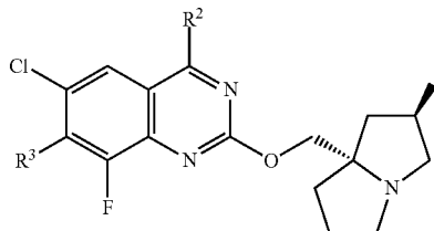
Formula II-1-B
