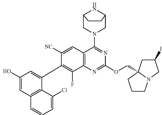
Atropisomer B
