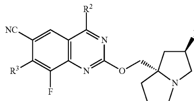
Formula II-2-B-E1
