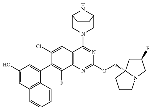
Atropisomer B
