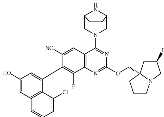
Atropisomer A
