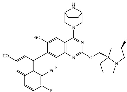
Atropisomer B
