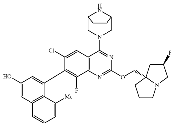
Atropisomer B
