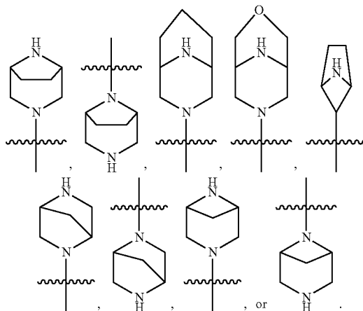
Formula I-1
