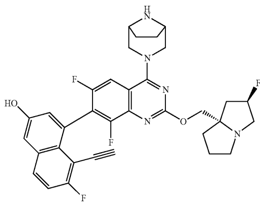
Atropisomer A
