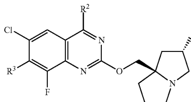
Formula II-2-B
