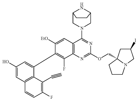
Atropisomer B
