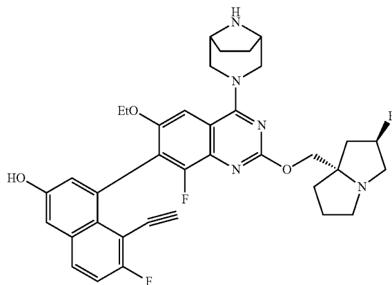
Atropisomer B
