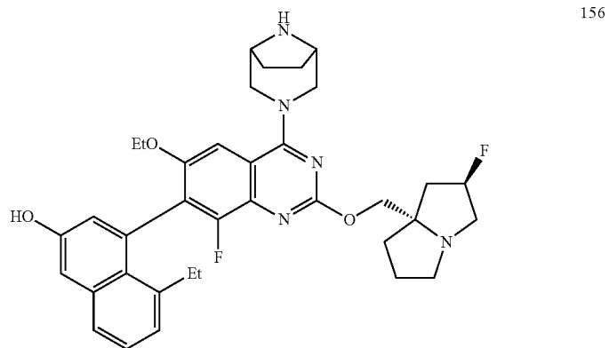
Atropisomer A
