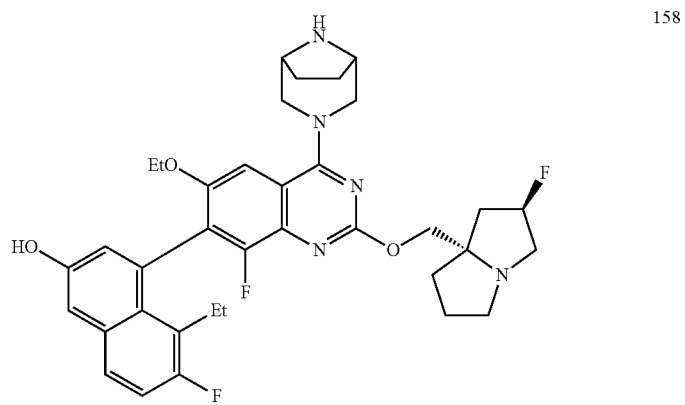
Atropisomer A
