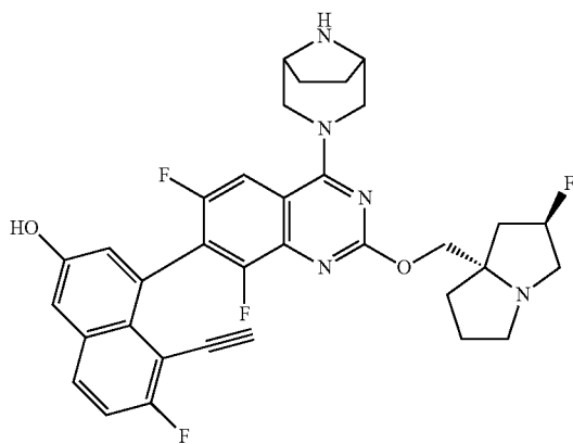
Atropisomer B
