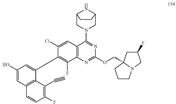
Atropisomer A
