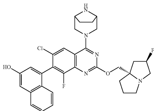
Atropisomer A
