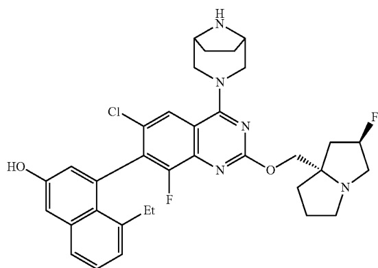
Atropisomer B
