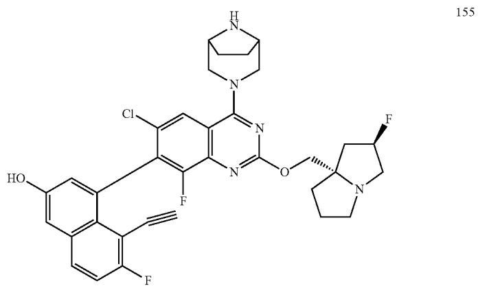
Atropisomer B
