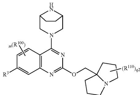
Formula I-1-A-3
