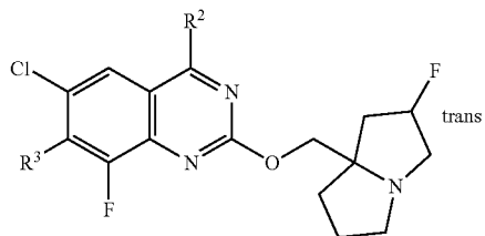
Formula II-2-B
