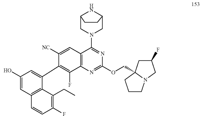
Atropisomer B
