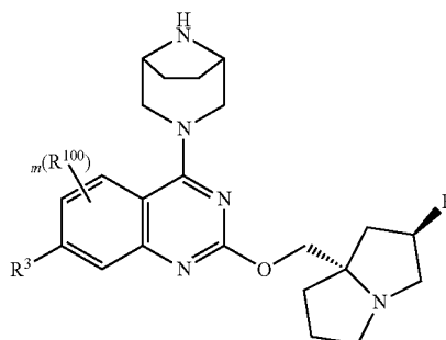
Formula I-1-A-4-E2
