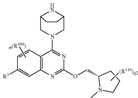
Formula I-1-A-3
