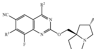
Formula II-2-B-E2
