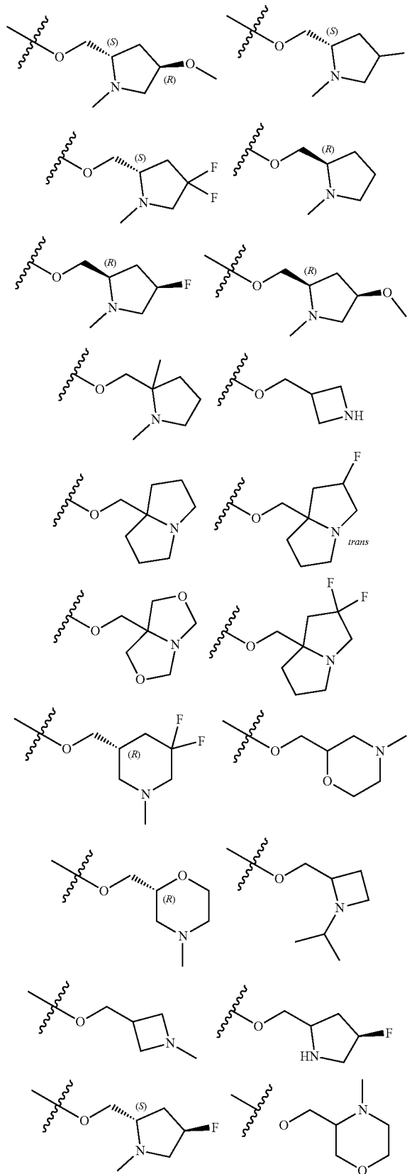
Formula III-9
