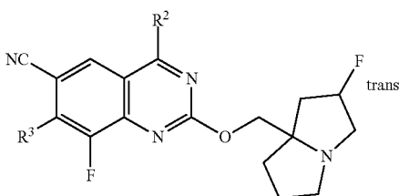
Formula II-2-C
