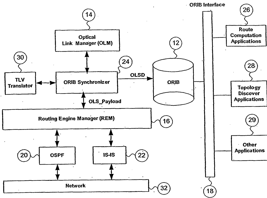
Figure 1: Generic ORIB Management Software Architecture
