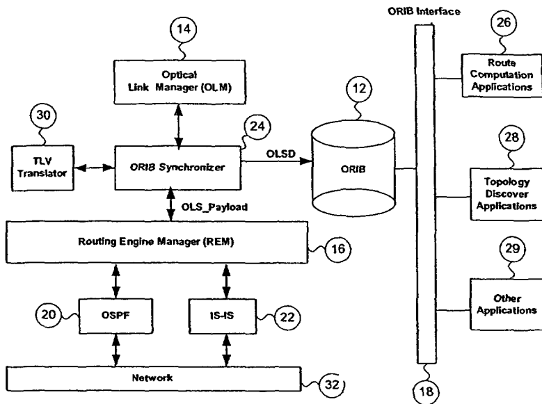
Generic ORIB Management Software Architecture
