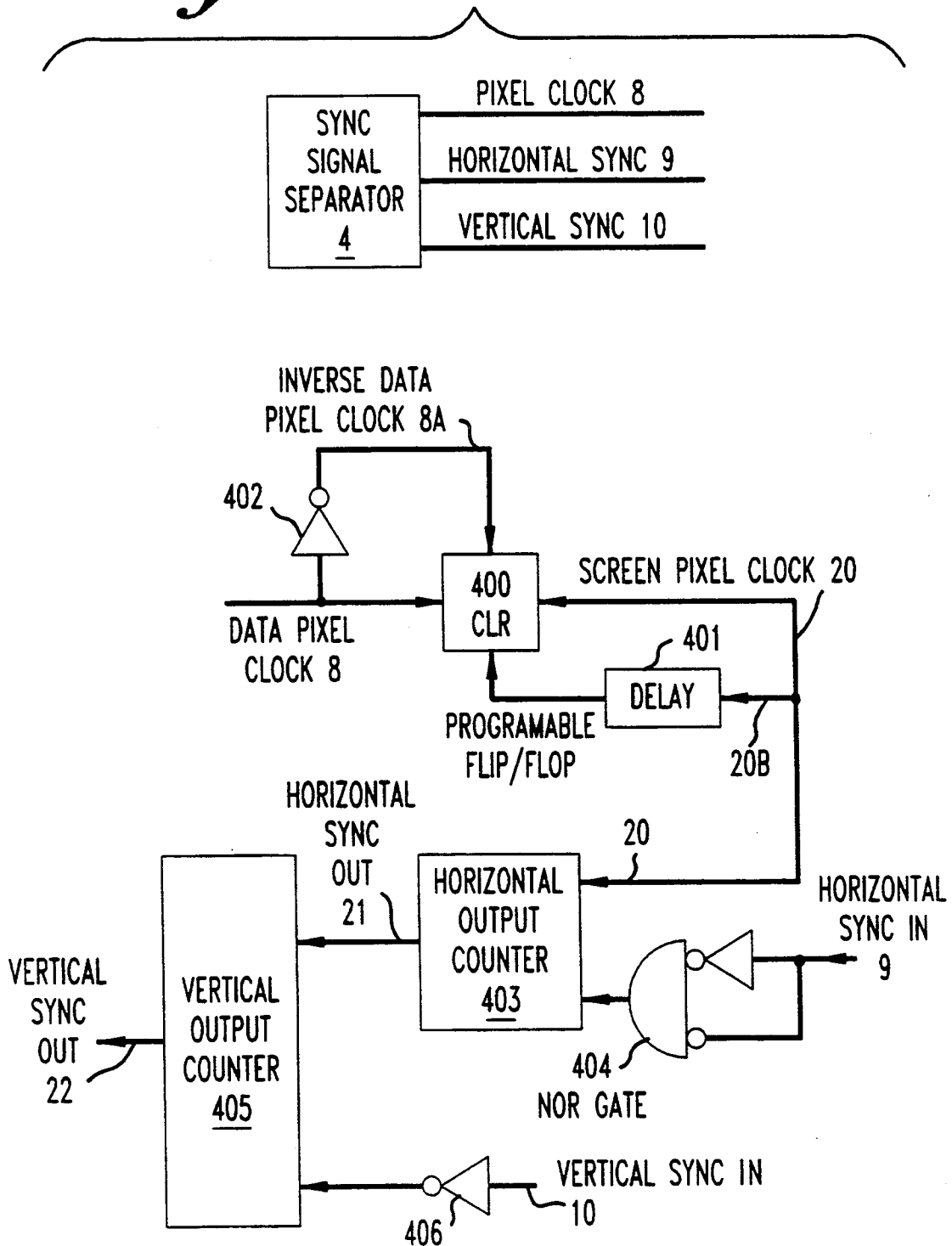
Fig. 5. CLOCK GENERATOR
