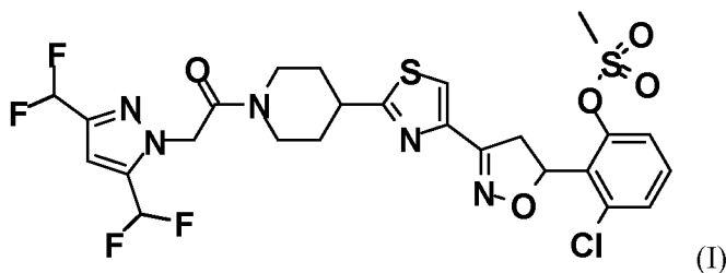
Figure 1: 2-{3-[2-(1-{[3,5-bis(difluoromethyl)-1H-pyrazol-1-yl]acetyl}piperidin-4-yl)-1,3-thiazol-4-yl]-4,5-dihydro-1,2-oxazol-5-yl}-3-chlorophenyl methanesulfonate
